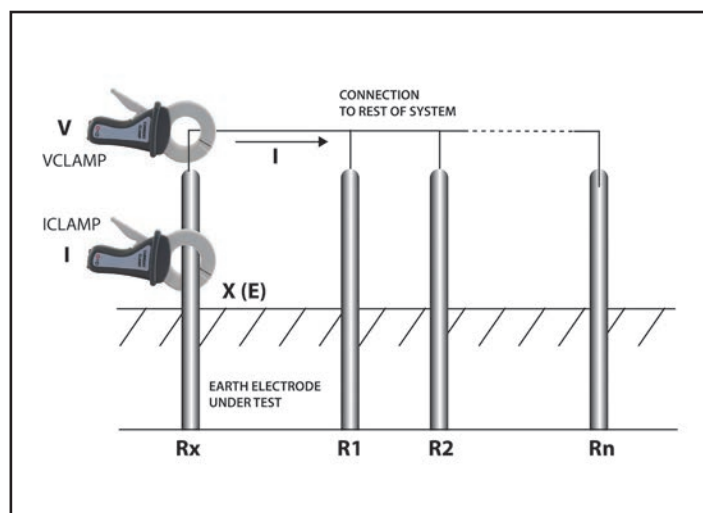
Schematic for two-clamp stakeless resistance measurement
