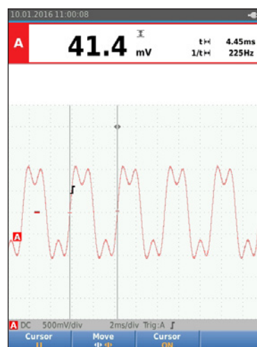
Evaluate period-to-period time changes.
