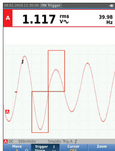
If the two components of the waveform are not symmetrical, there may be a problem with the signal.
