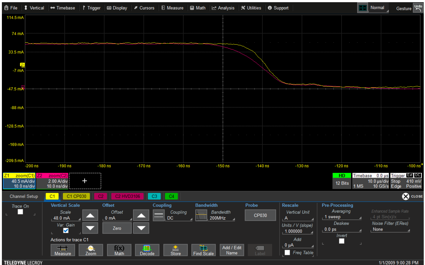
Voltage and current waveforms prior to deskew.
