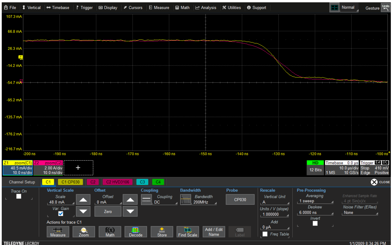
Voltage and current waveforms following deskew.
