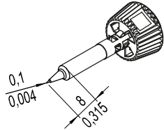
0142PDLF08/SB pencil point, 0.8 mm \phi
