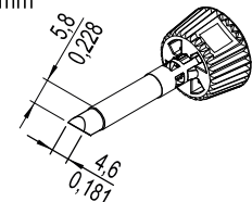
0142CDLF80A/SB chisel-shaped, asymmetric, 4.6 mm
