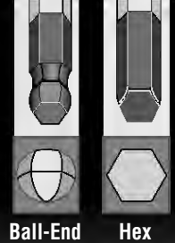
Ball-End
