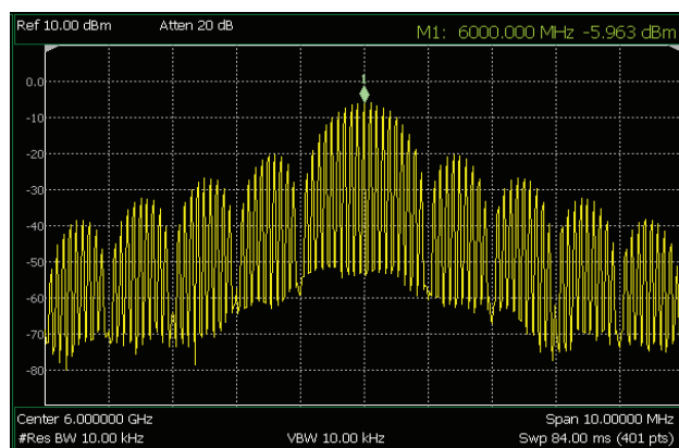
(b) Spectrum of a radar pulse
