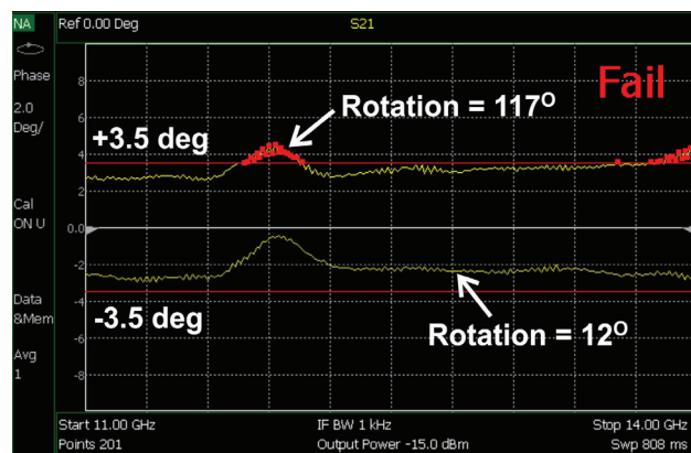
(b) S21 Phase
