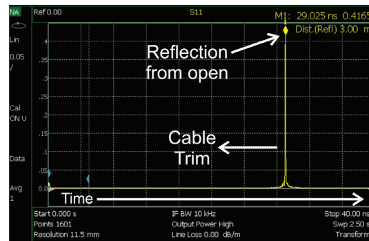
Figure 11. Measured time domain response from an open-ended cable using FieldFox VNA mode
