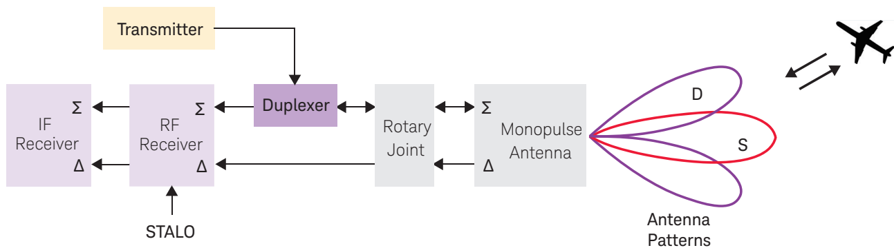
Figure 2. Simplified block diagram of a monopulse radar system
