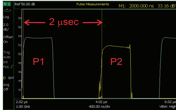
Figure 7. Measurement of ATCRBS transmitter P1/P2 timing offset
