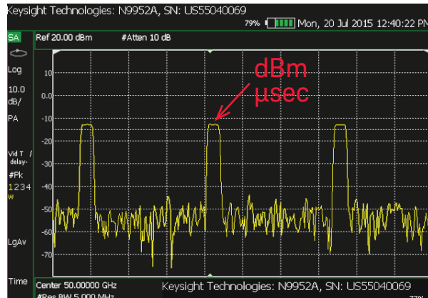
(a) Absolute time domain measurement using spectrum analyzer
