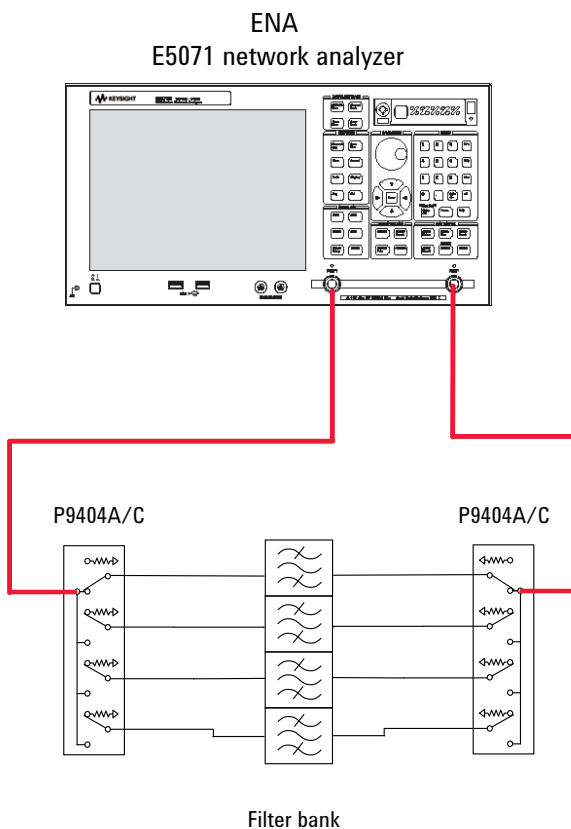
Figure 1. Filter bank test setup
