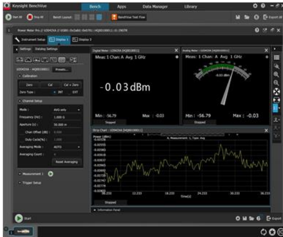
Figure 7. Digital Meter, Analog Meter and Datalog view
