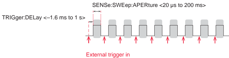
Figure 1. The X-Series power sensor offers real time measurement by measuring every consecutive pulse without dead time.
