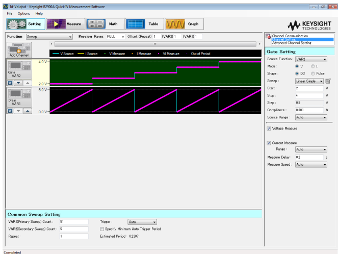
Quick I/V Measurement Software
