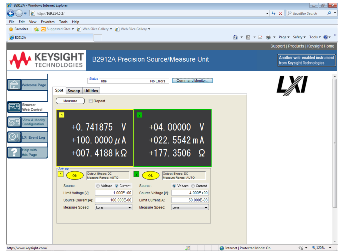
Graphical Web Interface
