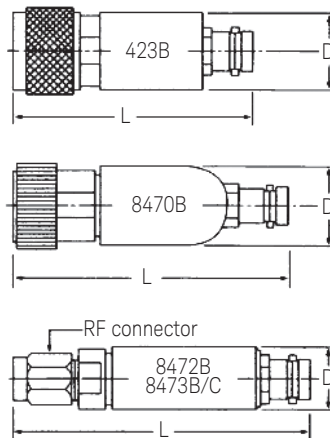
Figure 5. Drawing dimensions given in specification table
