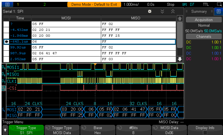
Figure 18: SPI trigger and decode.
