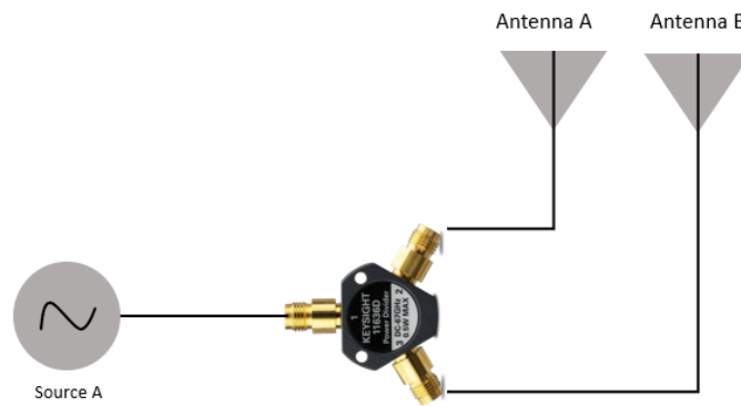
Figure 1. Test setup for power dividing application
