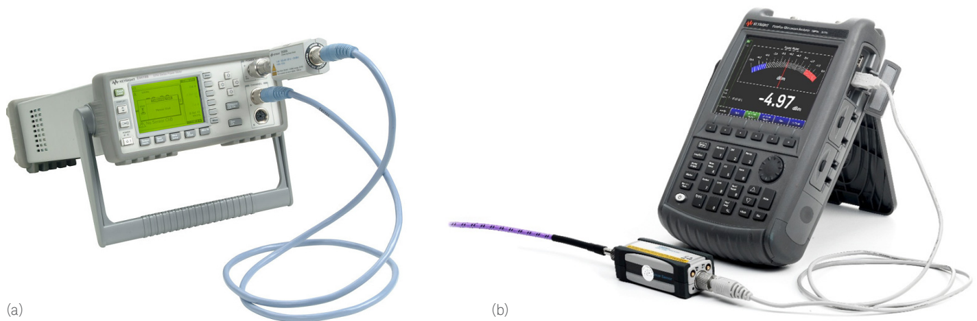
Figure 4. Equipment configurations for measuring RF power using a power sensor with the (a) power meter and (b) FieldFox
