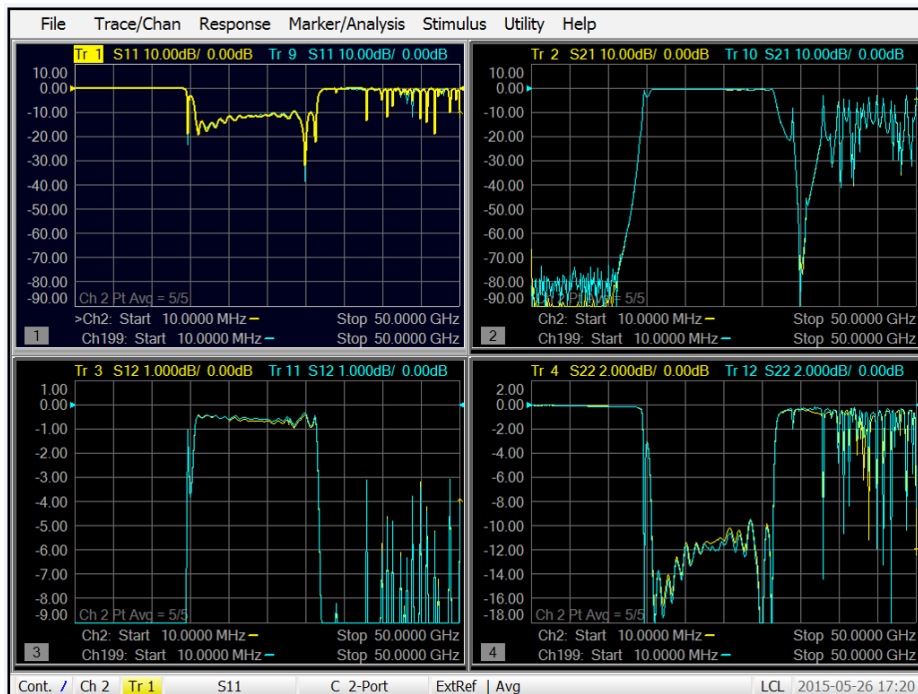
Figure 3. Measured S-parameters of a 15 to 30 GHz band pass filter; the plot overlays include measurements from a Keysight PNA-X (yellow) and FieldFox VNA (blue).
