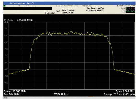
Figure 5. DDS versus Keysight's Trueform technology constellation and spectral diagram. In this figure, the same QPSK signal is generated by DDS and Trueform generators. The differences are significant in terms of modulation quality (EVM, error vector magnitude) and spectral quality (notice the 20-dB difference in dynamic range). The elliptical distribution of dots (in red) in the DDS constellation diagram shows jitter as phase noise in the modulation domain; pure noise (Gaussian noise) will make the constellation dots be circular in shape, as can be seen on the Trueform generator output. Spectral growth is a consequence of the sample jitter produced by the DDS architecture.
