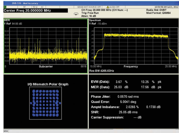
Figure 9. OFDM signal generation not only requires good waveform generator performance, but it often requires long record lengths, as well. This DVB-T signal (8K mode) requires several MSamples to store the minimum 68 OFDM symbols necessary to carry the TPS information receivers need to properly demodulate the signal.
