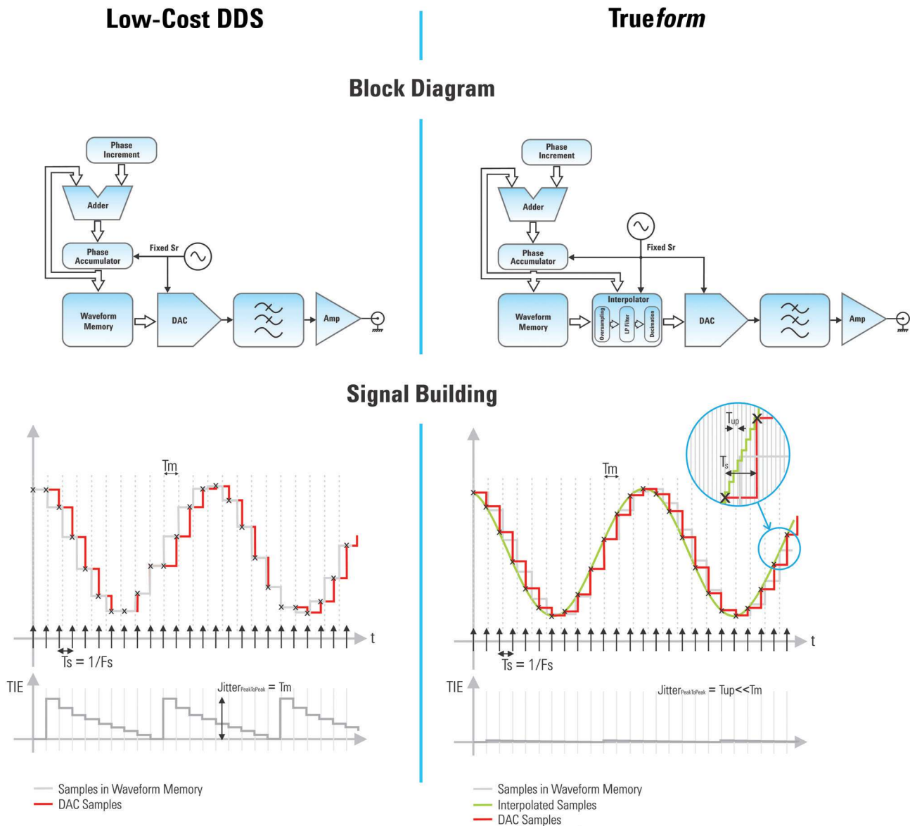
Figure 4. DDS versus Keysight's Trueform technology. The way traditional DDS architectures (left) access waveform memory results in an unacceptable level of jitter for modulated signal generation. Keysight's new Trueform architecture (right) eliminates the jitter, as the signal stored in memory is filtered, interpolated, and resampled in real-time.
