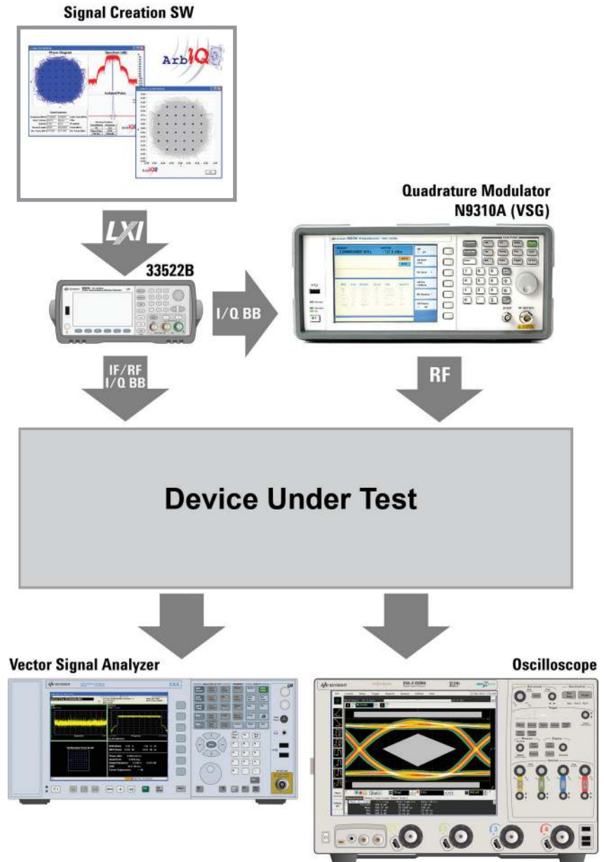
Figure 3. AWGs can generate RF modulated signals through two basic methods. Two-channel instruments can generate I and Q baseband signals that can be applied to an external quadrature generator. Single-channel instruments with sufficient sampling rate can directly generate a modulated carrier at IF or even RF frequencies.
