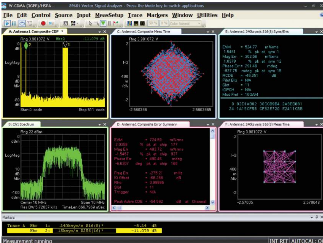
Figure 10. A 3GPP (UMTS) WCDMA downlink IF signal generated by a Keysight 33522B waveform generator. This is a complex signal, since it carries different data and synchronization channels.
