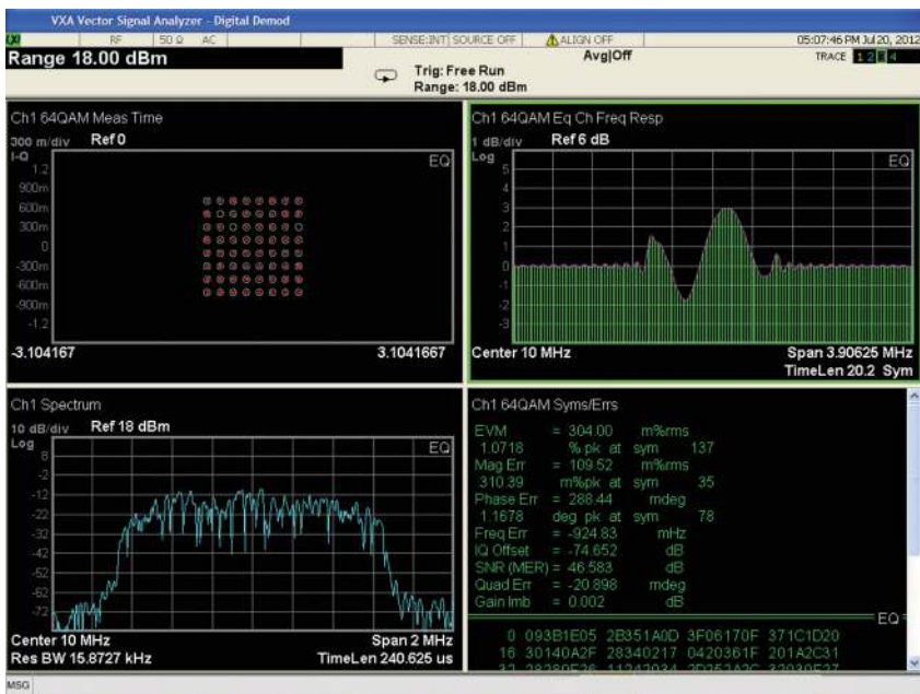
Figure 8. Modulation and spectral quality define the performance of any modulated signal generator. The ability to simulate linear and non-linear distortions caused by transmission equipment and the signal path is also important. In this figure, a radio-link 64QAM with multipath distortion is generated using a Keysight 33522B waveform generator. The adaptive equalizer in the Keysight CXA analyzer (top right) shows the corresponding channel response. Modulation quality for the corrected signal is excellent (0.3%).
