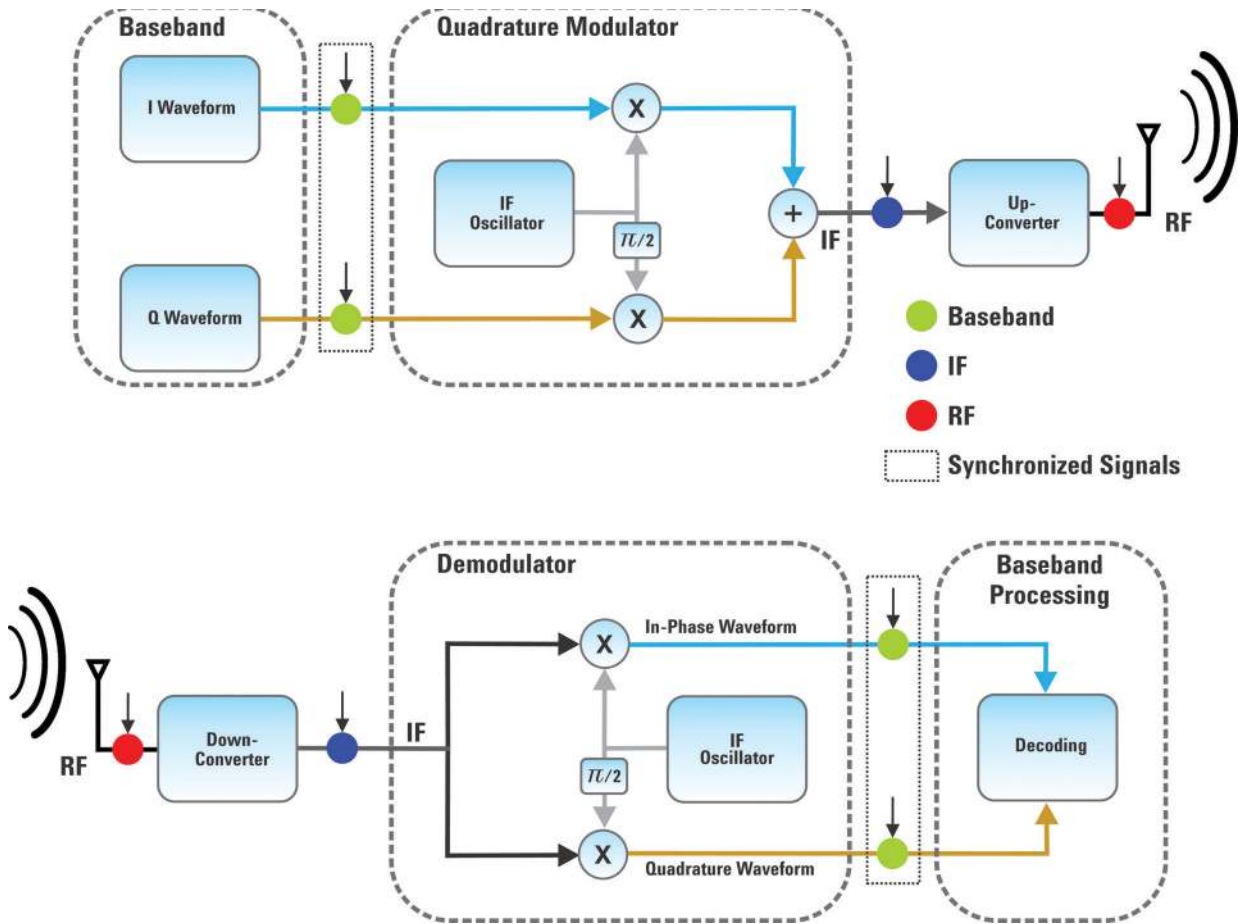
Figure 1. Simplified block diagram of a digital wireless system. Most modern modulation schemes are based on quadrature modulation, in which two orthogonal carriers transport portions of a digital message. This figure also shows where signal generators can be applied during transmitter and receiver testing.
