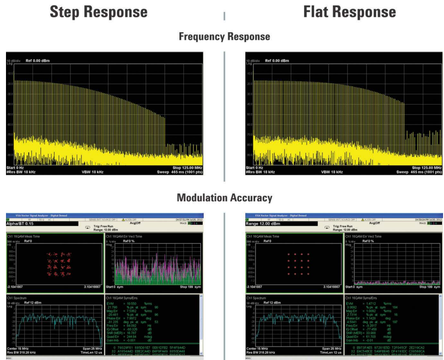
Figure 6. Trueform architecture can optimize the waveform generator frequency response for flatness or step response. Regular AWGs are typically optimized for step response. In this figure, a 100-tone signal covering the range from 1 MHz to 100 MHz has been used to assess frequency response in both filter modes (top). Generating a 20-MBaud 16QAM signal and analyzing its quality in the two modes shows the importance of flat response for high-quality wideband modulation generation (bottom). With a sampling rate of 250 MHz and the Trueform signal generation technique, the usable digital bandwidth is much larger than it is with other forms of generation, which can be normalized with software for flatness as high as 100 MHz.
