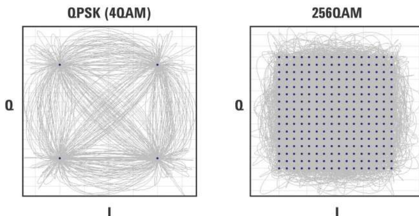
Figure 2. Phase/constellation diagrams are a convenient way to show modulation schemes. They are basically an I versus Q Cartesian representation that directly translates to a polar (magnitude versus phase) representation of the carrier state of modulation. In this figure, constellations (blue dots) of QPSK and 256QAM modulations are shown. While QPSK carries just two bits per symbol, 256QAM carries six bits per symbol, although the bigger distance between different symbol locations makes QPSK more resilient to noise or lower-accuracy components.
