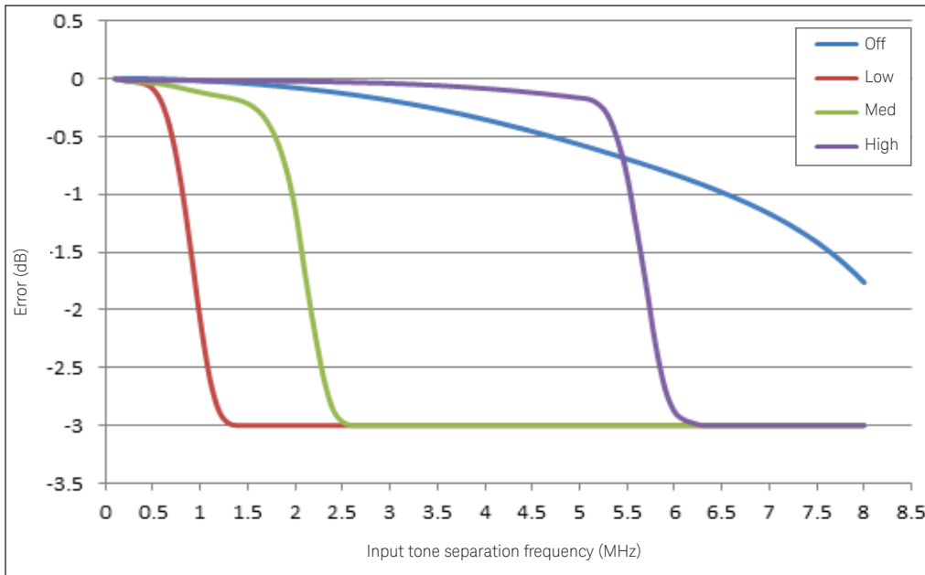
Figure 7. U2042/44/49XA and L2065XT error in peak-to-average ratio measurements for a two-tone input (High, Medium, Low and Off video bandwidth settings).
