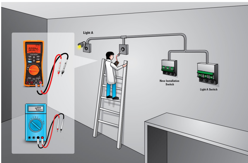
Figure 1. Electrician detects stray voltage on the unused connection with high input impedance multimeter (shown in blue).
