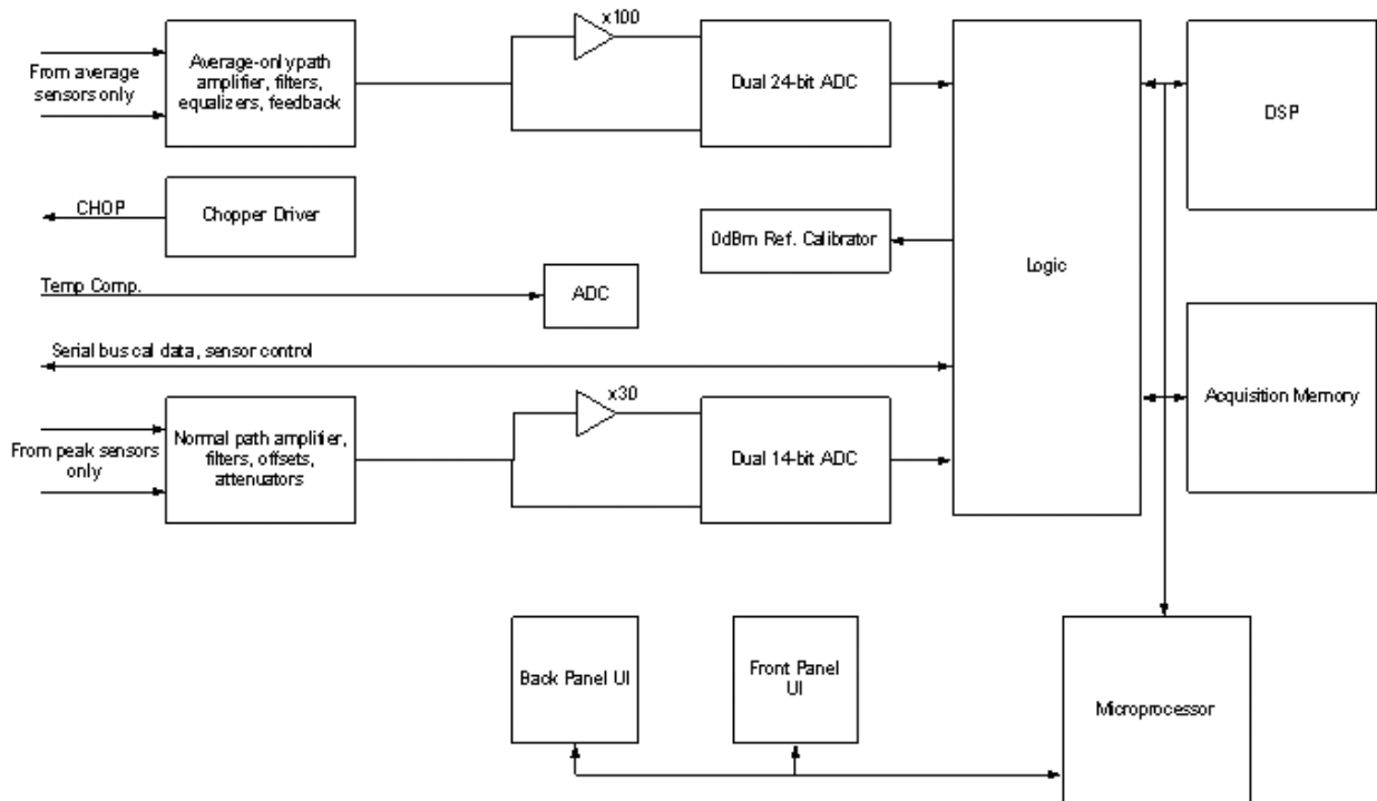
Figure 5-17. P-Series power meter simplified block diagram
