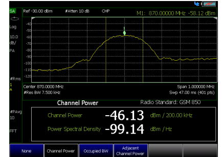
Channel power measurement
