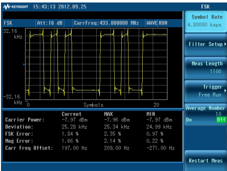
Viewing FSK demodulation metrics with option DMA
