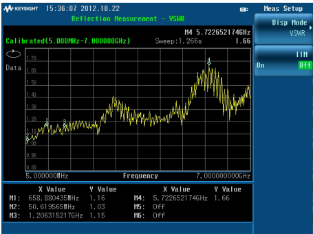
Using the option RM7 for reflection measurements
