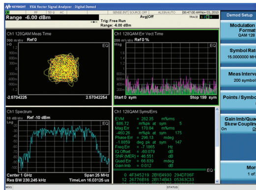
Figure 3. W9064A VXA vector signal analysis measurement application
