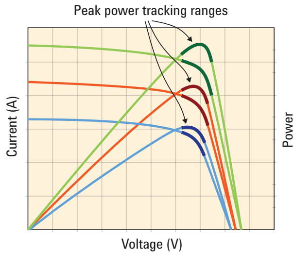
Peak power tracking with a range of illumination and power tracking range
