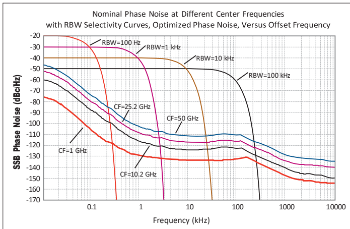
Figure 3. Nominal PXA phase noise at various center frequencies with standard LO.
