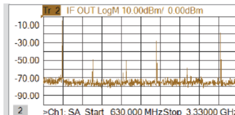
Output spectrum on IF port
