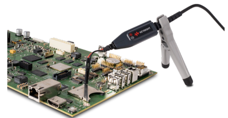
DP001xA Series probe using socketed Y-lead
