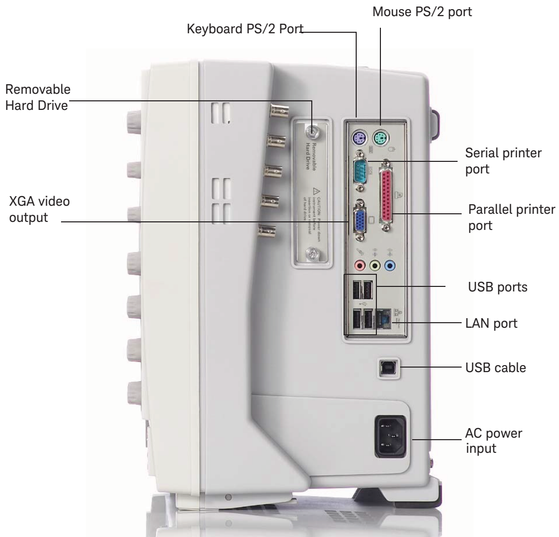
Figure 2 Side panel
