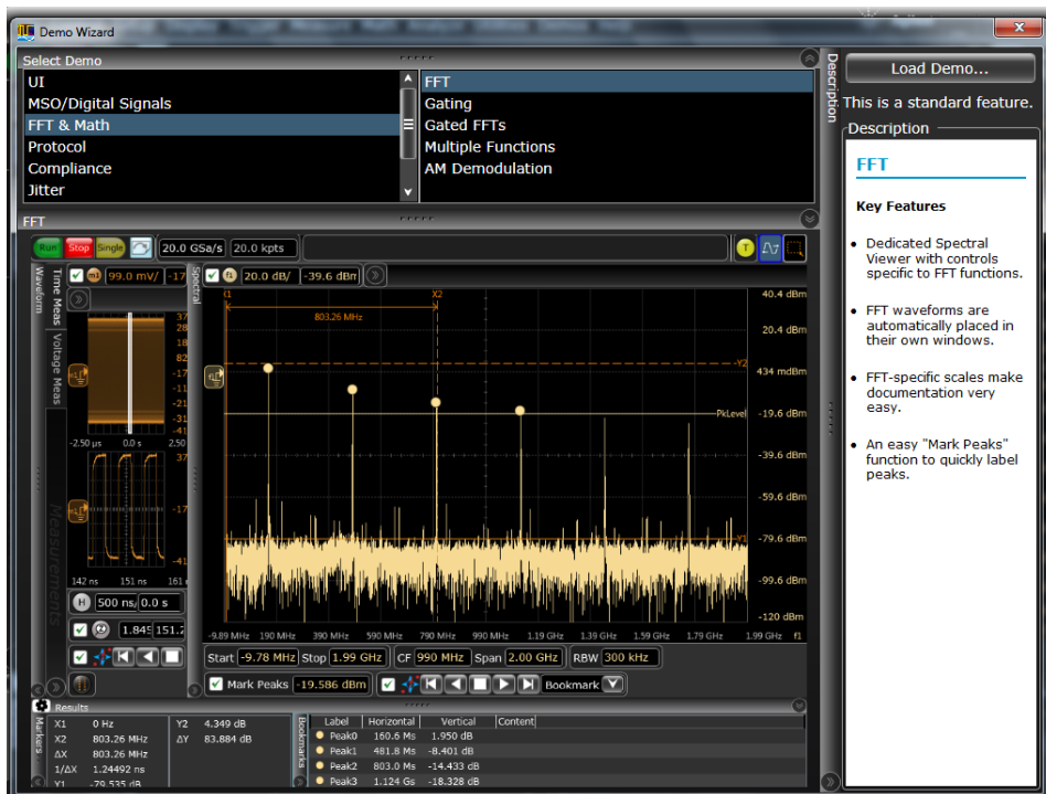
Figure 24 FFT Demo
