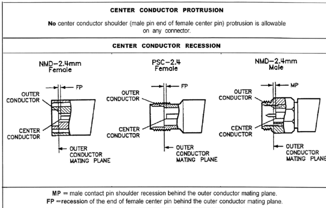
Figure 1 85130G Specifications
