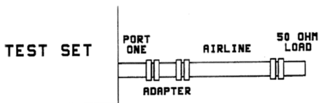
Figure 2 Return Loss Setup
