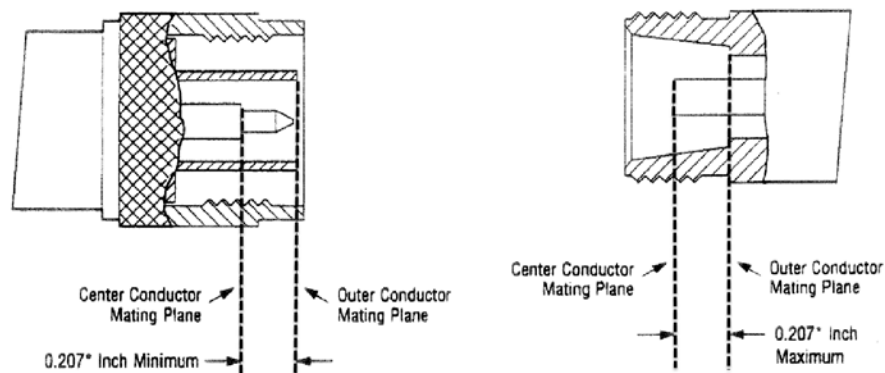
Figure 1 Type-N Connectors
