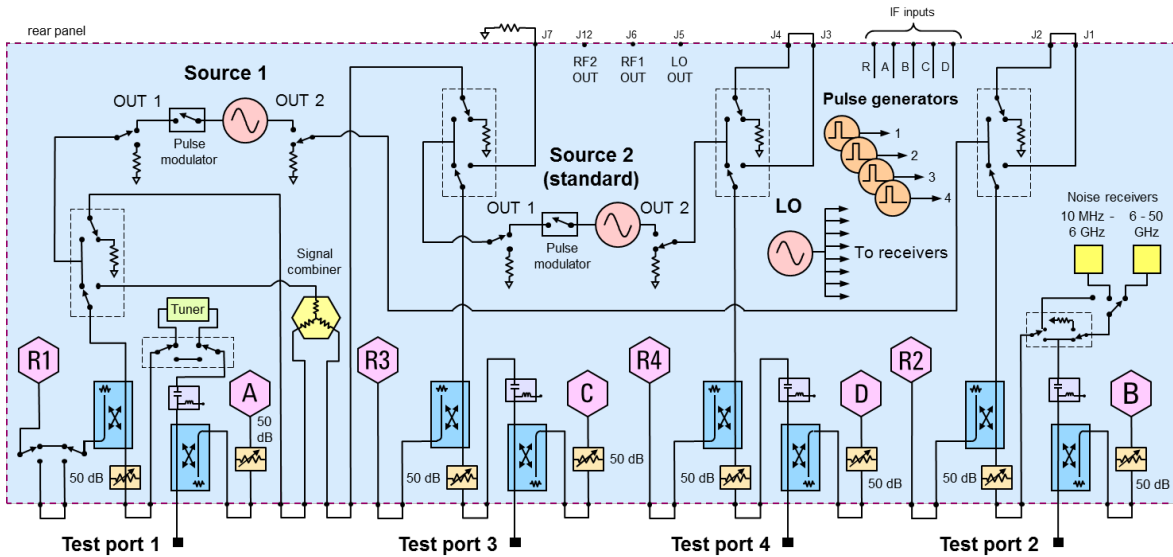
Figure 9. 4-Port N5247B Option 423 with 029
