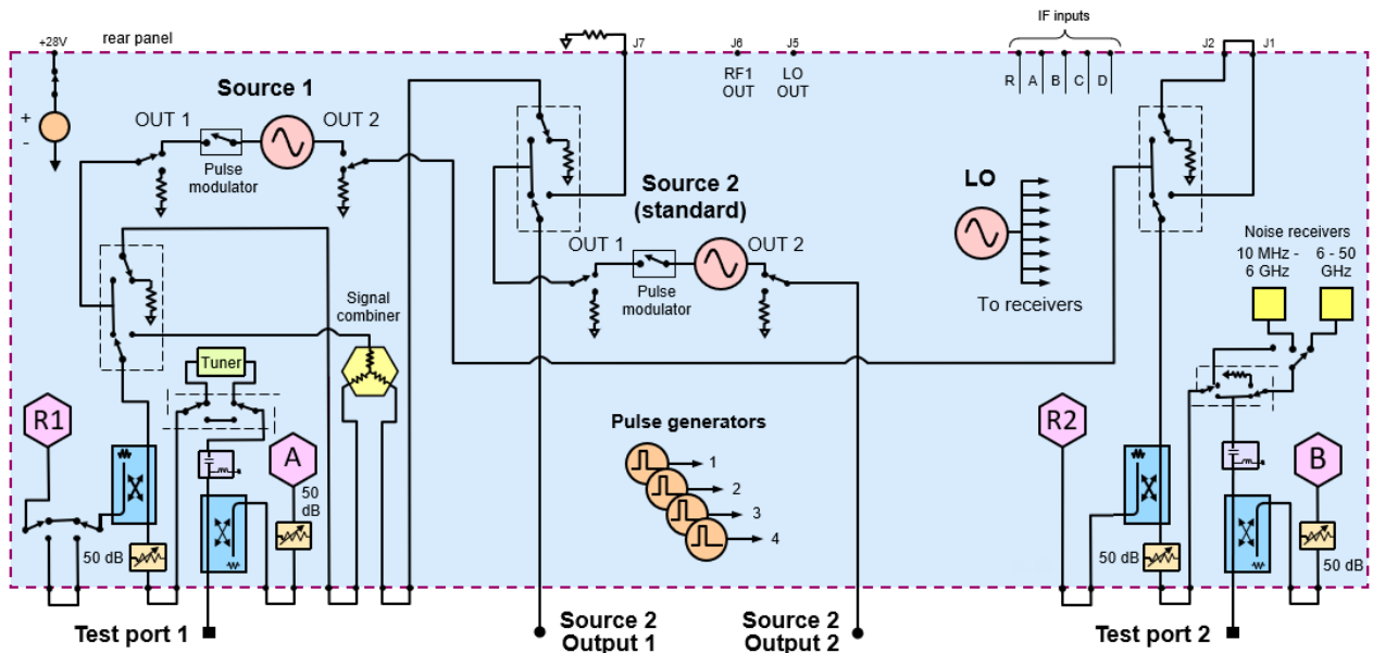
Figure 4. 2-Port N5247B Option 224 with 029
