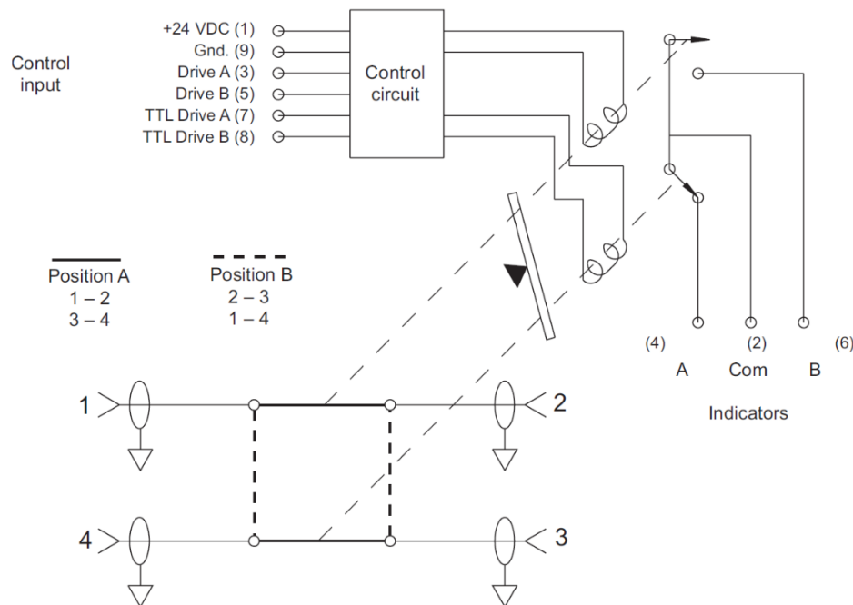
Figure 1. Keysight 87222C/D/E schematic
