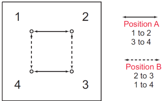
Figure 7. RF port connections
