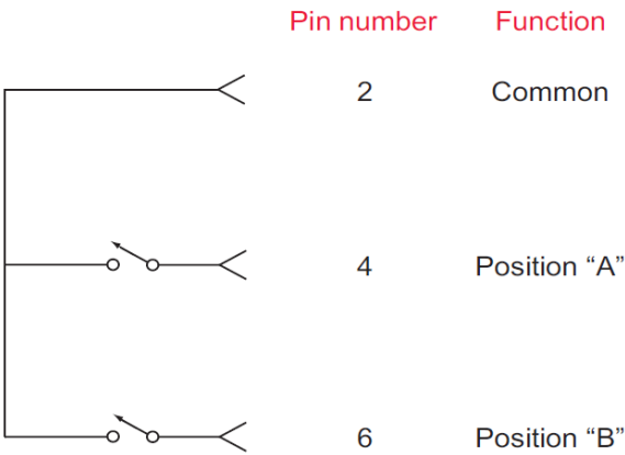
Figure 10. Indicator function diagram
