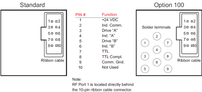
Figure 8. Drive connections
