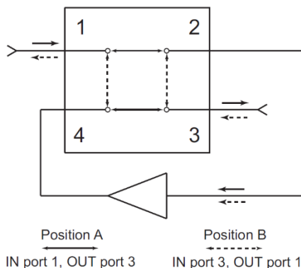
Figure 4. Signal reversal
