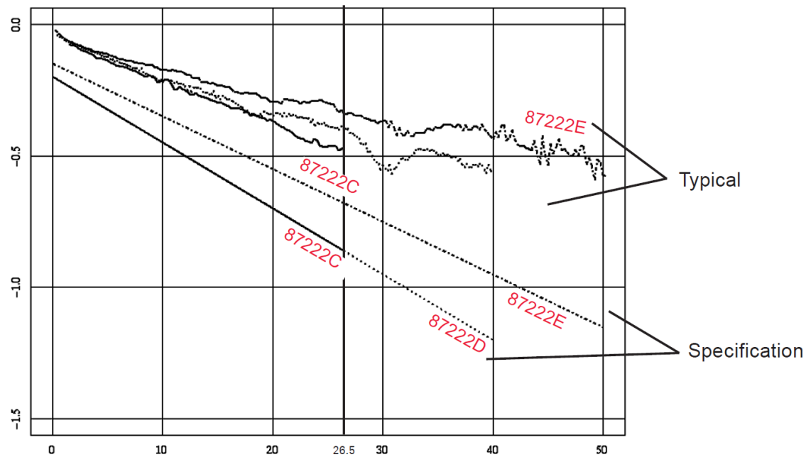
Figure 11. Keysight 87222C/D/E insertion loss versus frequency
