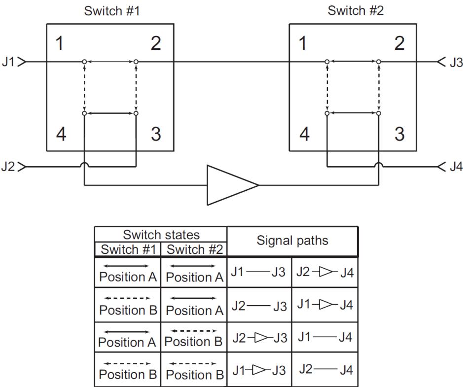
Figure 6. Bypassing an active device
