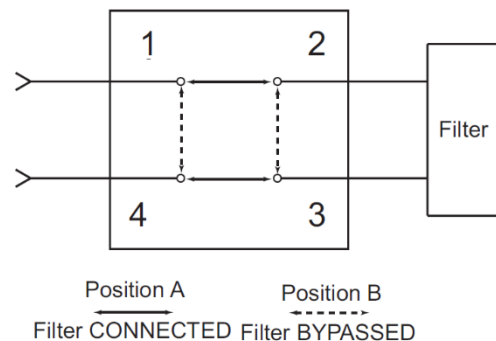
Figure 3. Drop-out switch
