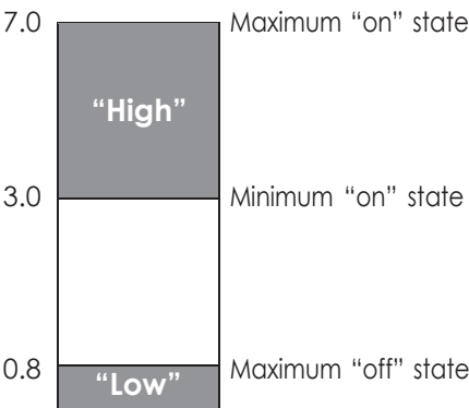
Figure 8. TTL control voltage states (Option T24)
