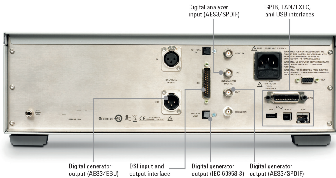
Figure 8. U8903A audio analyzer, rear view
