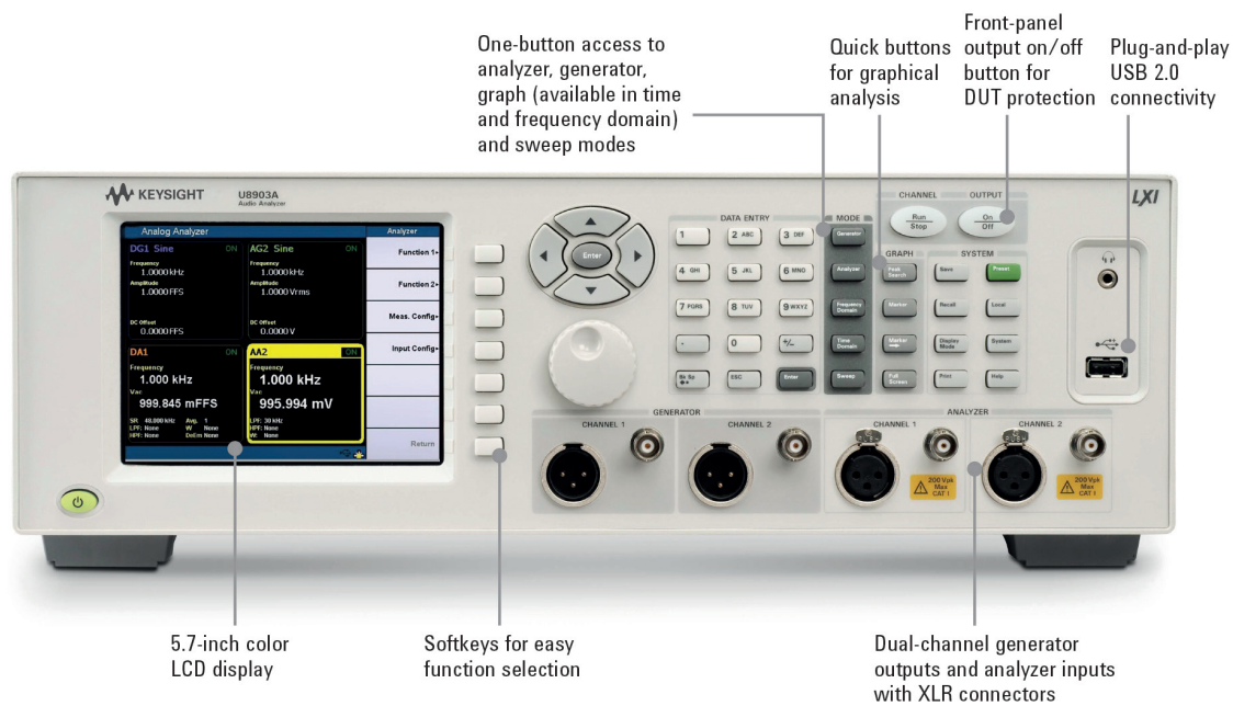
Figure 7. U8903A audio analyzer, front view
