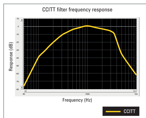
Figure 17. CCITT filter frequency response
