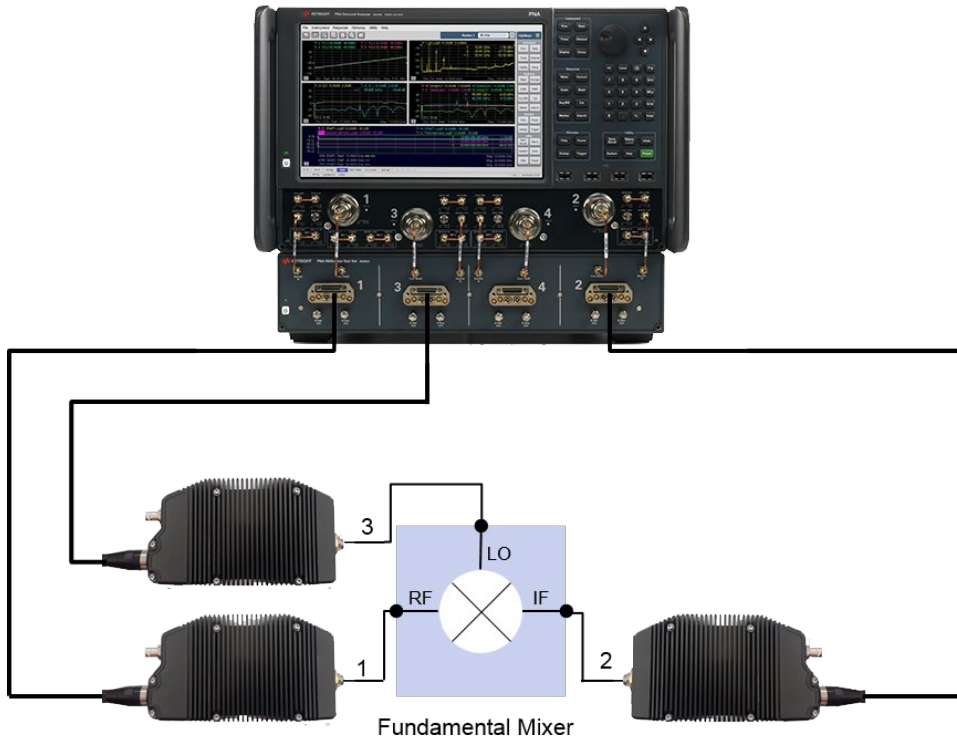
Figure 34. A dual-source PNA with an N5292A four-port controller and broadband frequency-extender modules characterize mixers and converters at millimeter wave frequencies. The PNA's second source can be used to provide an LO signal to a mixer.
