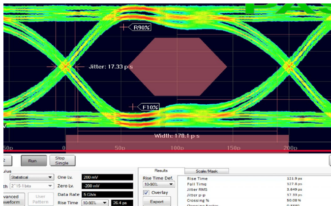
Figure 28. The simulated eye diagram analysis capability eliminates the need for a pulse pattern generator.
