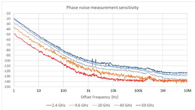
Figure 12. PNA Phase noise measurement noise floor
