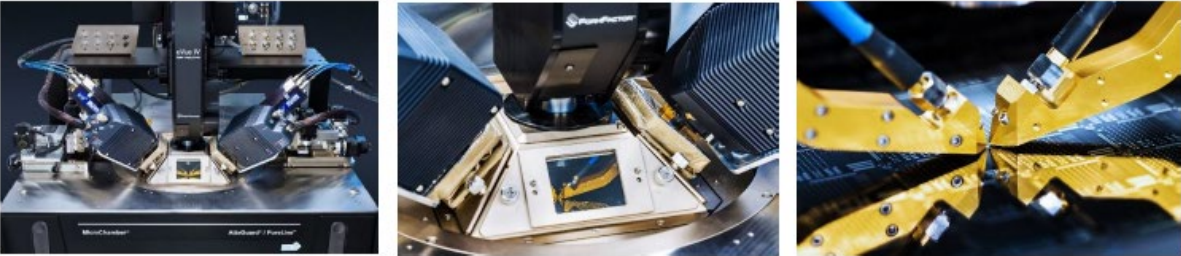
DMPI T-Wave Dual Probe, offered by Form Factor Inc.
