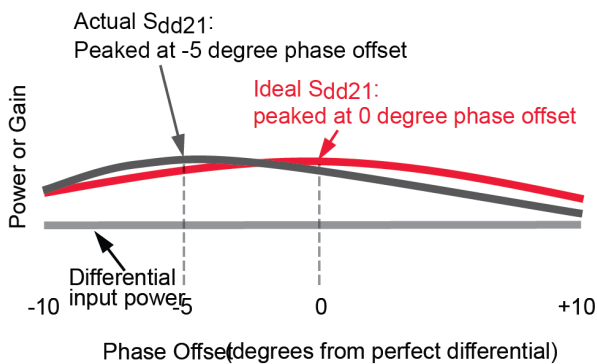
Figure 26. In-fixture phase-offset sweeps reveal the optimal phase offset to achieve the highest amplifier gain, which is essential to the design of the input matching circuit.
