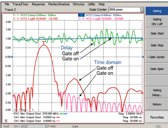
Figure 7. Time-domain gating can remove ripple by removing unwanted, time-delayed responses due to spurious signals.
