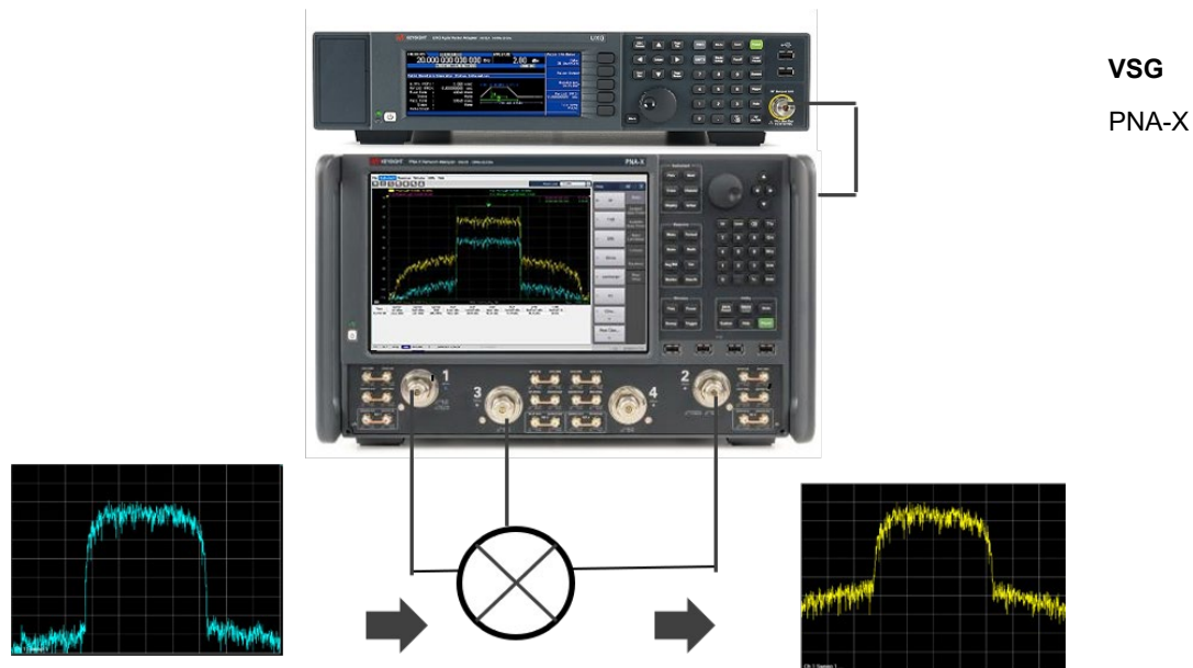
Figure 19. Mixer EVM/NPR/ACPR measurement with Modulation distortion application
