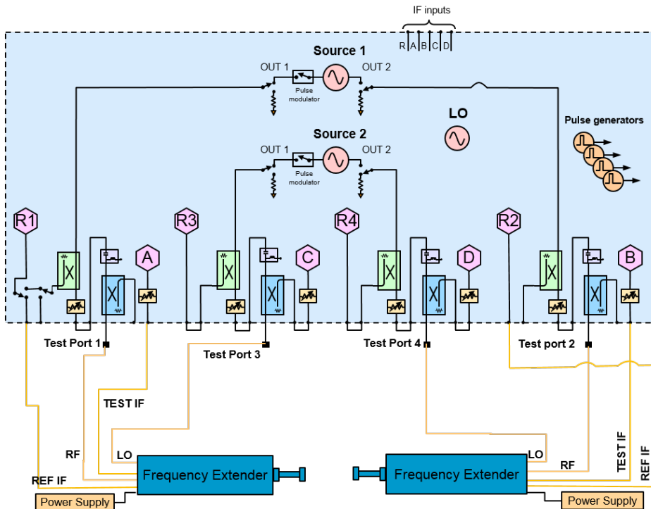
Figure 32. Block diagram of a two-port millimeter-wave system using a four-port PNA and two millimeter-wave frequency extenders.
