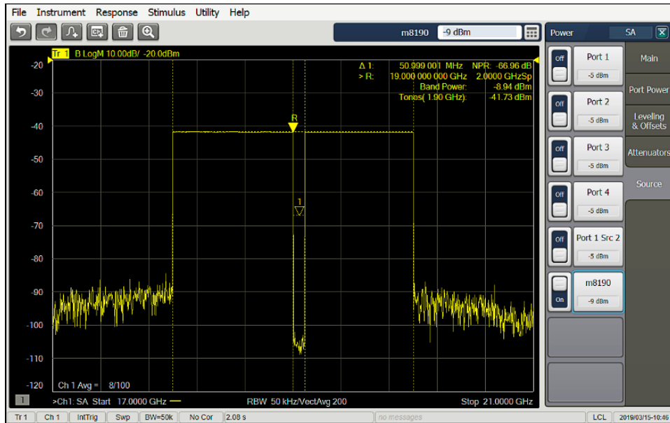
Figure 15. Improved flatness and lower noise floor in the notch after signal correction
