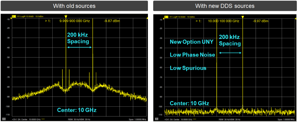
Figure 4. Two-tone measurements
