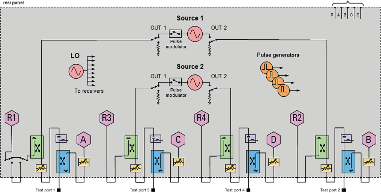
PNA Series block diagram shown with test set Option 419, plus pulse and external-IF options.
