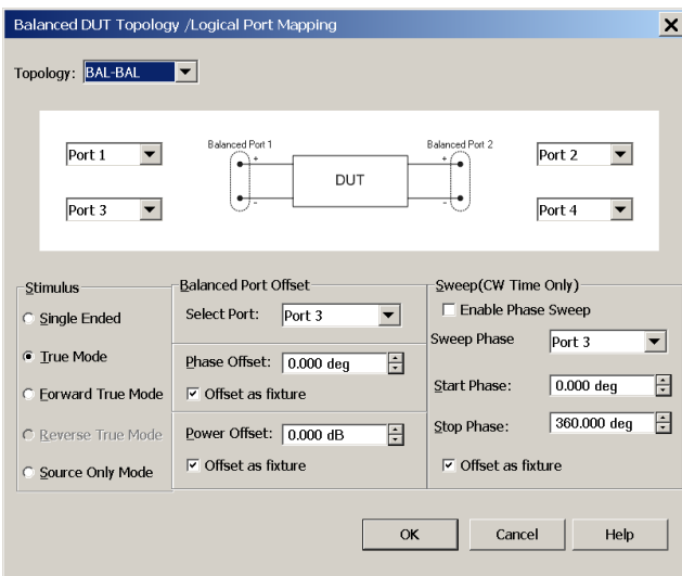
Figure 25. Various stimulus and sweep settings are available in the Balanced DUT Topology dialog, allowing you to select the right configuration for all of your balanced devices.
