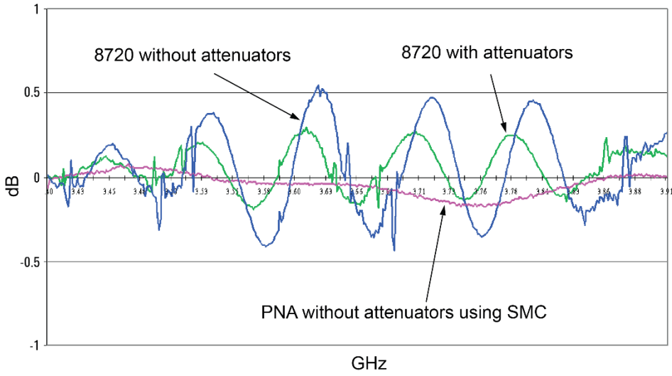
Figure 8. SMC's match correction greatly reduces mismatch errors in conversion loss/gain measurements, eliminating the need for attenuators at the ends of the test cables.
