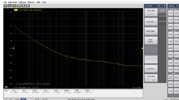
Figure 11. Oscillator phase noise, AM noise, and spurious measurement example
