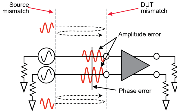
Figure 22. Without mismatch correction, the delivered signals to the DUT will not be truly differential due to reflection from the DUT input and the subsequent re-reflection from the sources. This effect can be corrected with mismatch correction.
