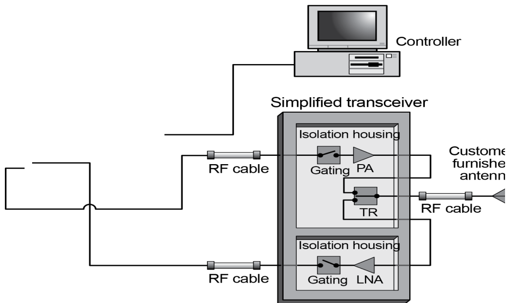
Figure 36. PNA-X configured for radar cross-section measurements 089
