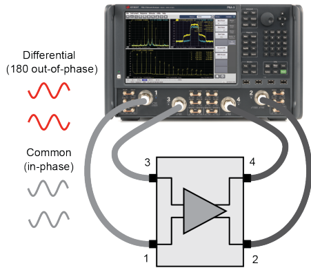
Figure 20. Using the PNA-X's two internal sources, iTMSA drives the differential amplifier under real world conditions, providing accurate mixed-mode S-parameters in all operating environments.
