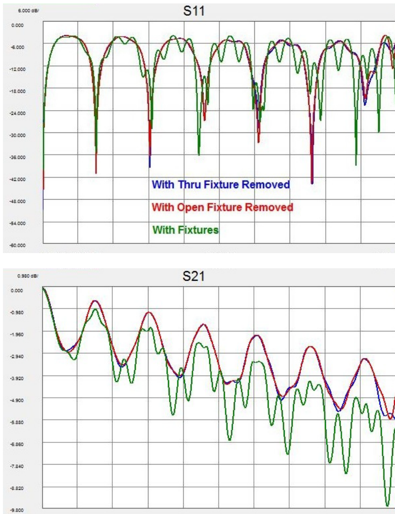
Figure 30. S11 and S21 in frequency domain
