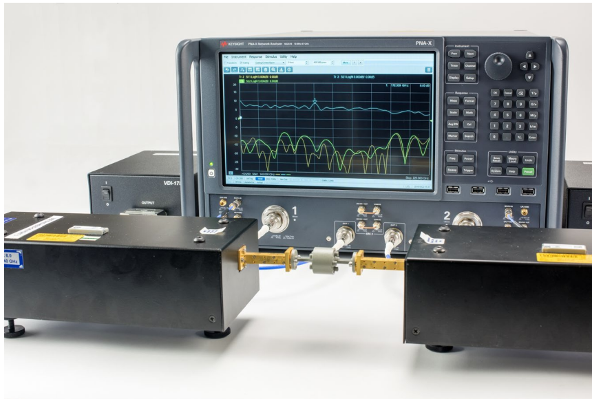
Figure 31. Direct connection of VDI modules to a four-port PNA-X enables S-parameter measurements to 1.5 THz.
