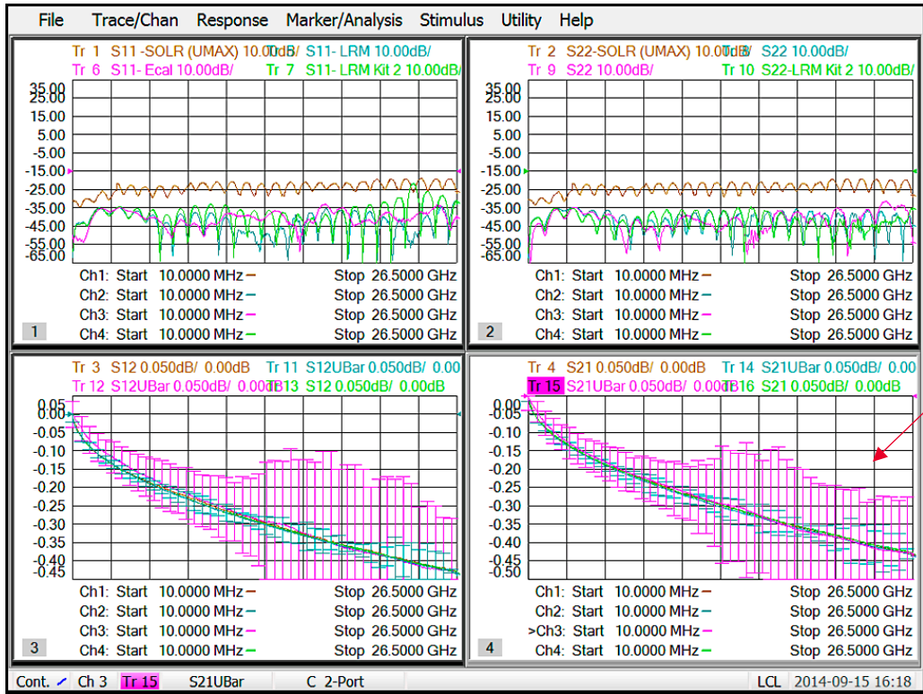
Real time uncertainty with measurement traces and uncertainty bars
