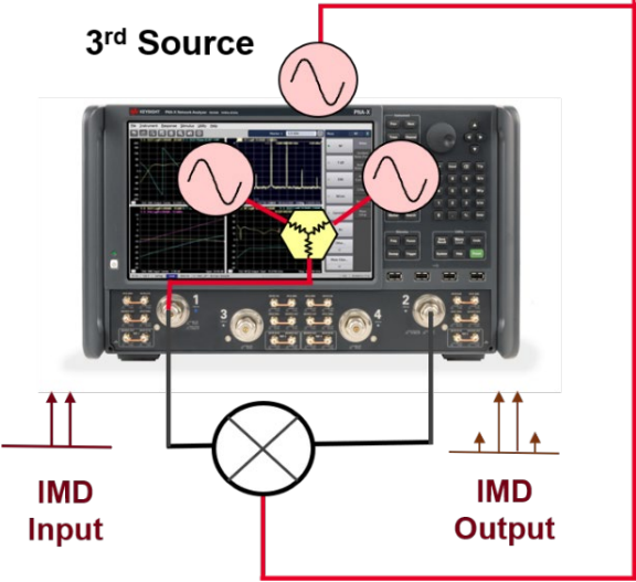
Figure 5. Two-tone IMD mixer measurement
