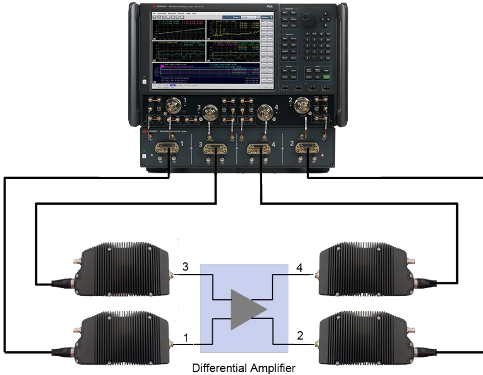
Figure 35. True-differential measurement of a balanced trans-impedance amplifier using a four-port PNA, the N5292A controller, and N5293A frequency extenders.
