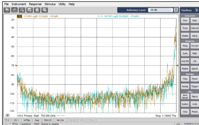
Figure 33. 100 dB dynamic range 750 GHz to 1.1 THz (IFBW = 10 Hz)
