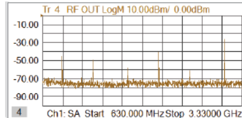
Output spectrum on RF port
