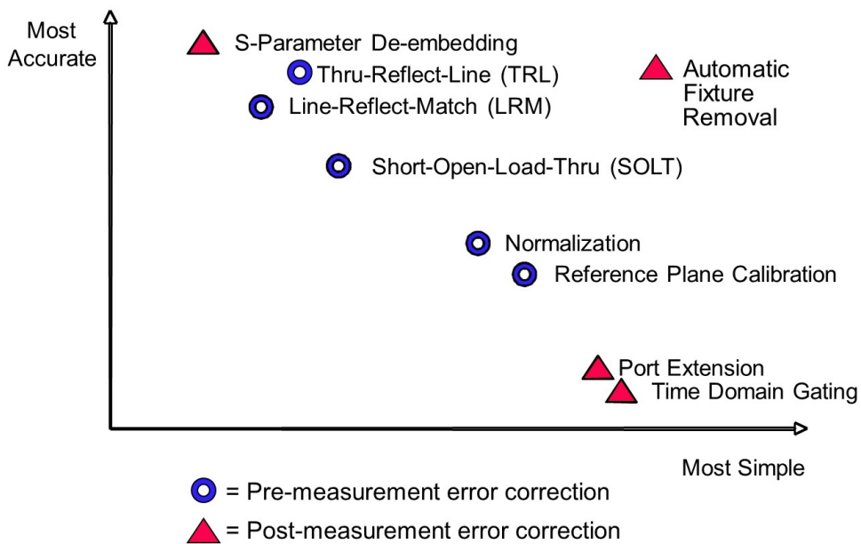
Figure 29. A relative comparison of various fixture error-correction methods
