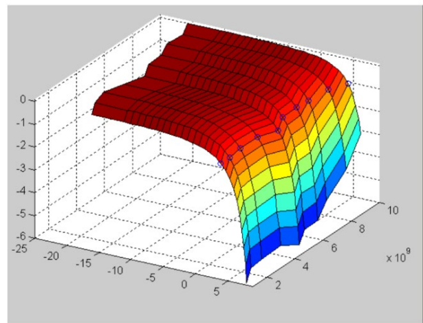
Complete device response to 2D sweeps — gain versus frequency and power — can be extracted for device modeling.
