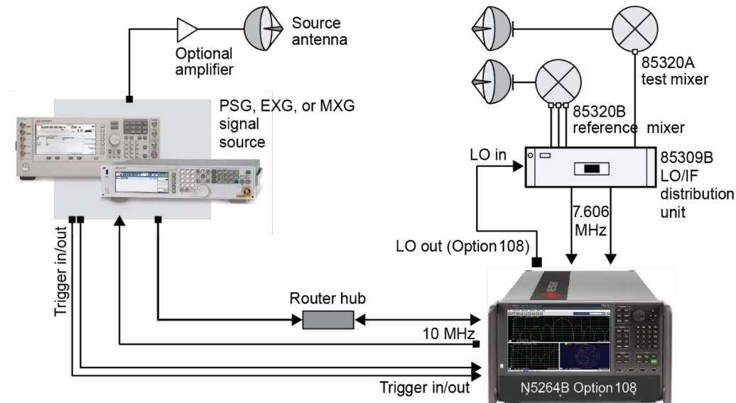
Figure 38. PNA-X measurement receiver configured for far-field measurements (PNA-X Option 020 with IF inputs can also be used).
