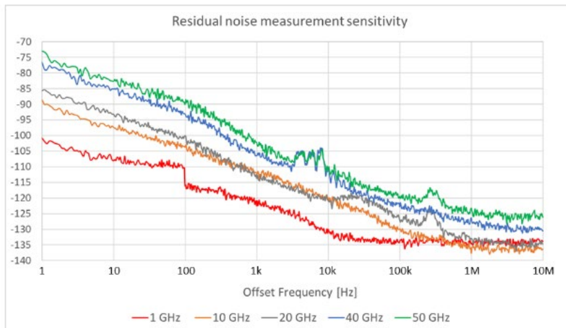
Figure 13. PNA residual noise measurement noise floor
