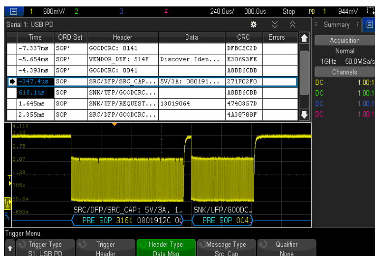
Figure 3. USB PD decode on an InfiniiVision X-Series
