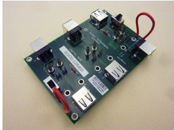
Figure 6. E2626B “SQuIDD” test fixture for testing USB 2.0 low- and full-speed products.
