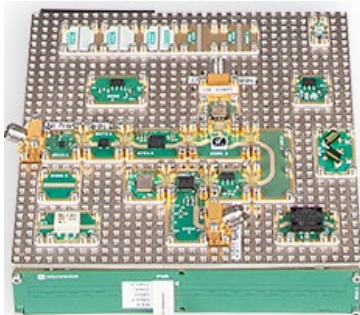
Figure 4: Prototype plate
