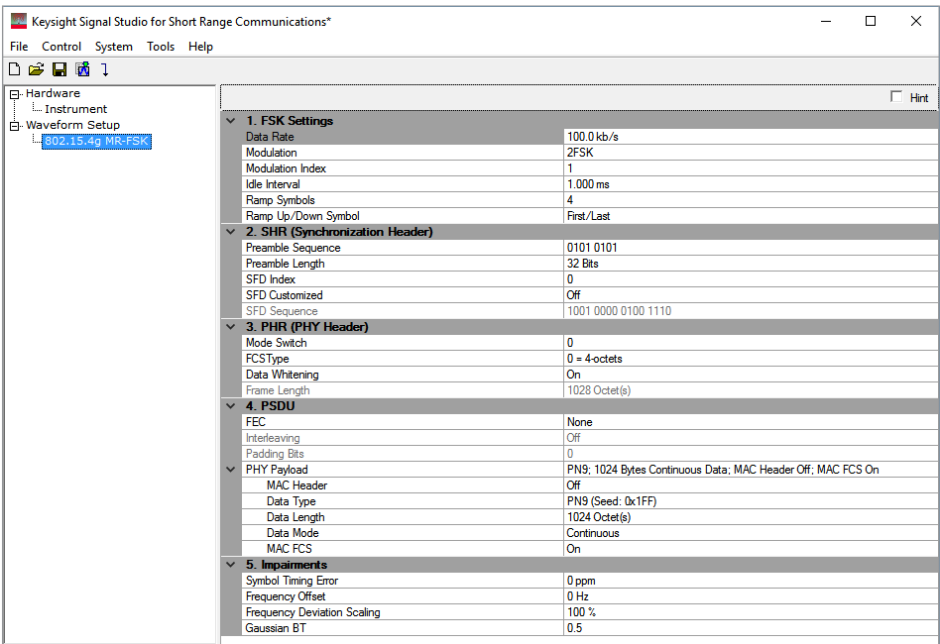
Figure 3. Wi-SUN MR-FSK configuration user interface
