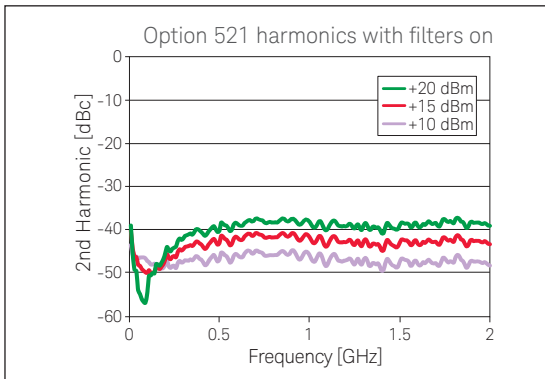
Harmonics (measured)
