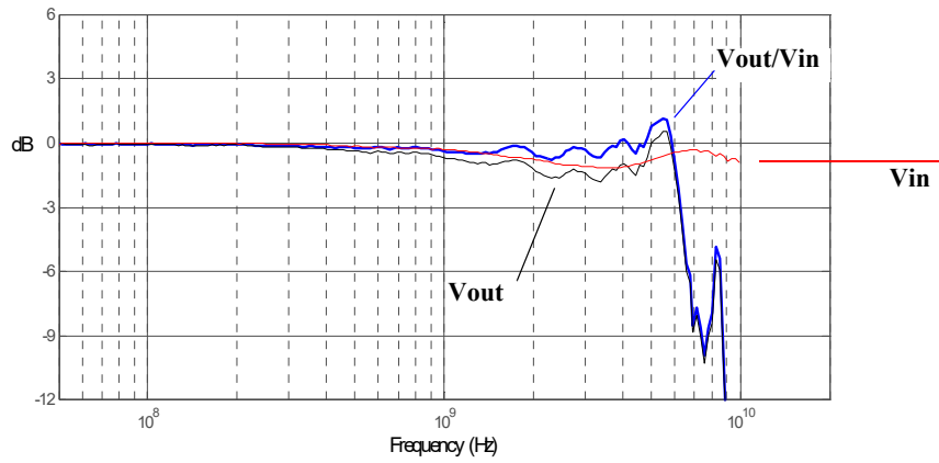
Figure 162 Graph of V_{in} and V_{out} of probe with a 25\Omega source and V_{out}/V_{in} frequency response.
