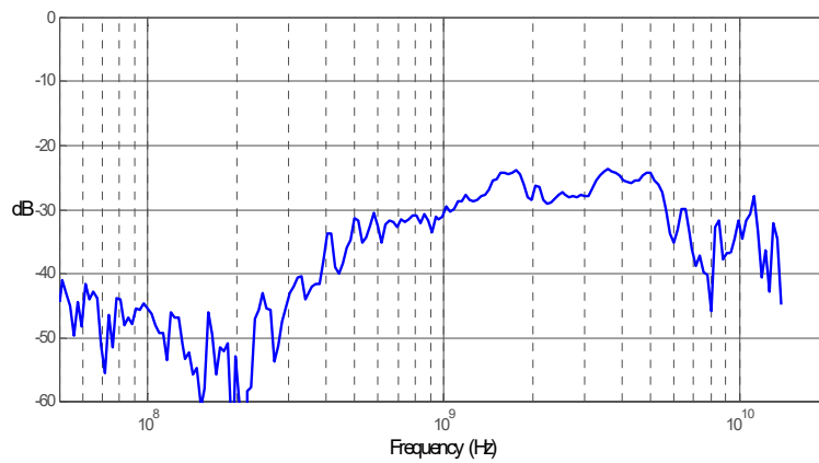
Figure 194 Graph of V_{out}/V_{in} frequency response when inputs driven in common (common mode rejection).
