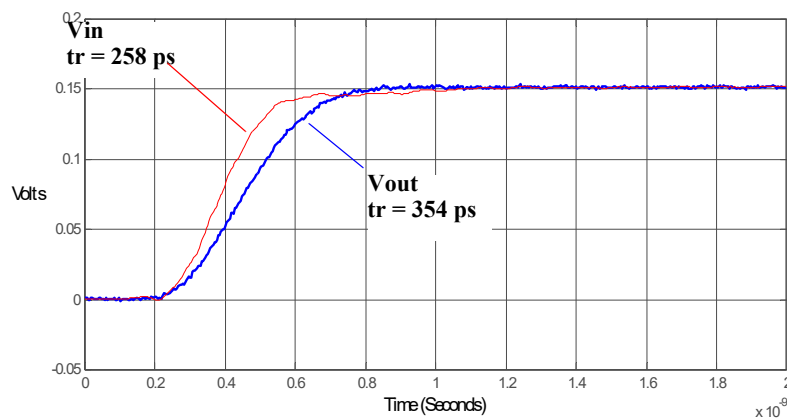
Figure 125 Graph of V_{in} and V_{out} of probe with a 25\Omega 240 ps step generator.
