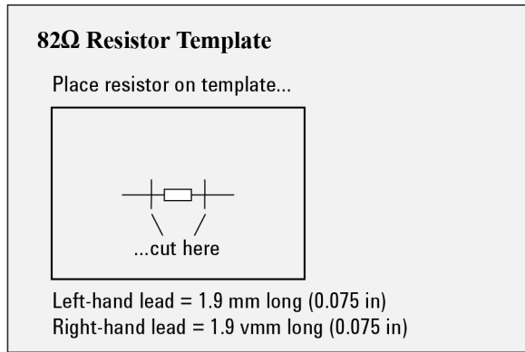
Figure 26 Resistor Trim Dimensions and Trim Guage
