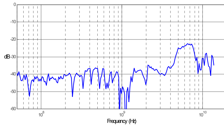
Figure 209 Graph of V_{out}/V_{in} frequency response when inputs driven in common (common mode rejection).
