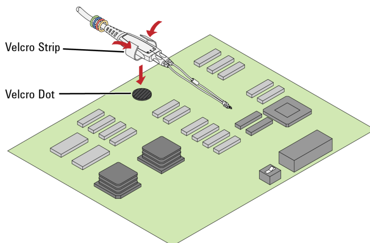
Figure 9 Using the Velcro Dots
