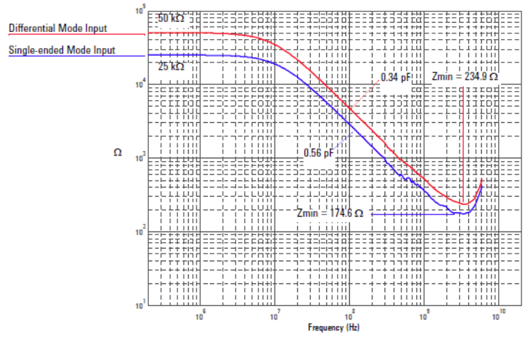
Figure 82 Magnitude plot of probe input impedance versus frequency.
