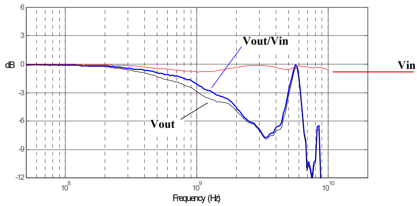
Figure 167 Graph of Vin and Vout of probe with a 25Ω source and Vout/Vin frequency response.
