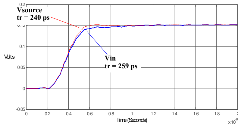
Figure 124 Graph of 25\Omega 240 ps step generator with and without probe connected.
