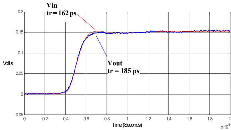
Figure 161 Graph of Vin and Vout of probe with a 25Ω 100 ps step generator.
