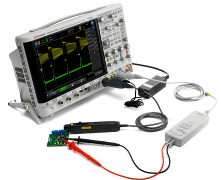
Figure 3. Clamp-on current probe is an indirect type of current sensing technique where the probe is clamped around the current carrying wire or conductor to make non-contact current measurement.
