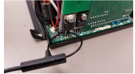
Figure 8. The lightweight clip-around sensor coil is flexible and easy to wrap around a current-carrying conductor.
