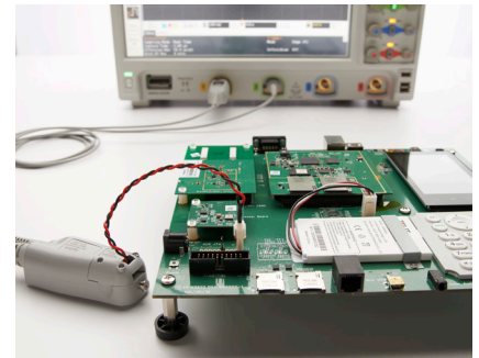
Figure 2. Keysight's N2820A/21A high sensitivity current probe utilizes sense resistor technology to measure low level current down to 500nA with an oscilloscope.
