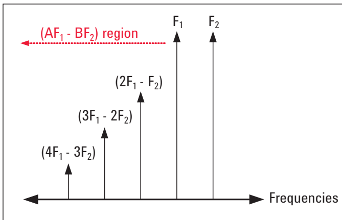
Figure 6. Intermodulation orders potentially affecting public safety
