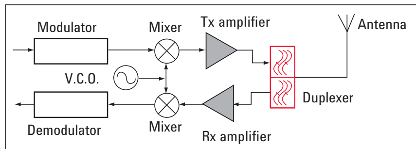
Figure 3. Block diagram of front end of analog radio
