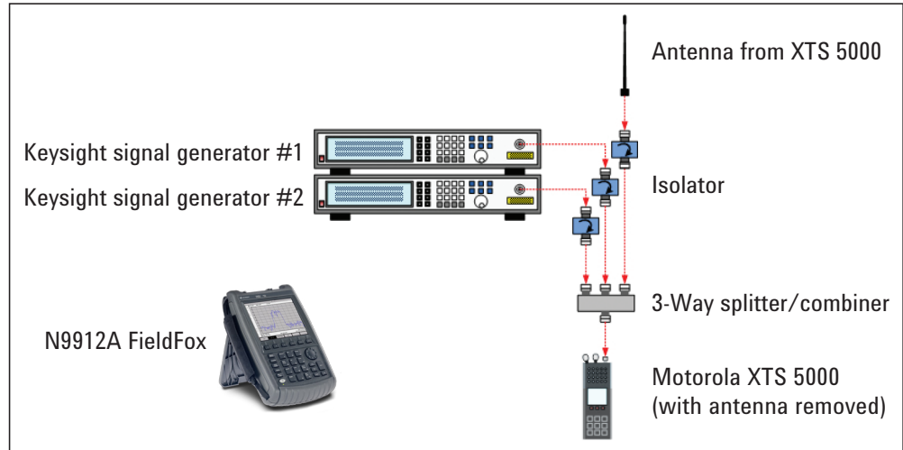
Figure 1. Block diagram of test setup
