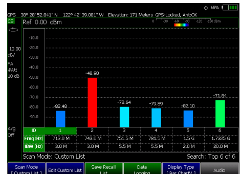
Scan up to 20 channel simultaneously with the channel scanner option
