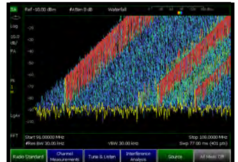
Waterfall display makes interference hunting easier
