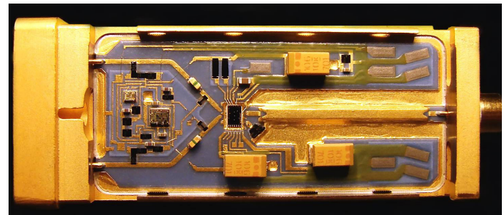
The Infiniium 30 GHz probing system uses the same InP technology that enables high bandwidth and low noise oscilloscope measurements.
