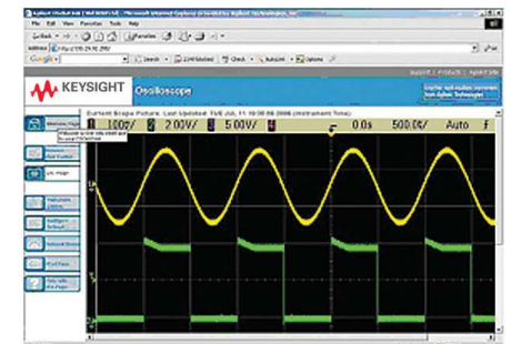
Remotely display and control your 6000L oscilloscope from any Java-enabled web browser over the oscilloscope's built-in LAN interface.
