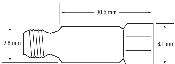
Figure 1. Outline drawing
