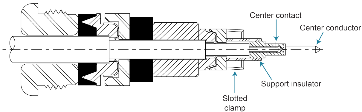
Figure 15: Add slotted clamp, support insulator, and center contact
