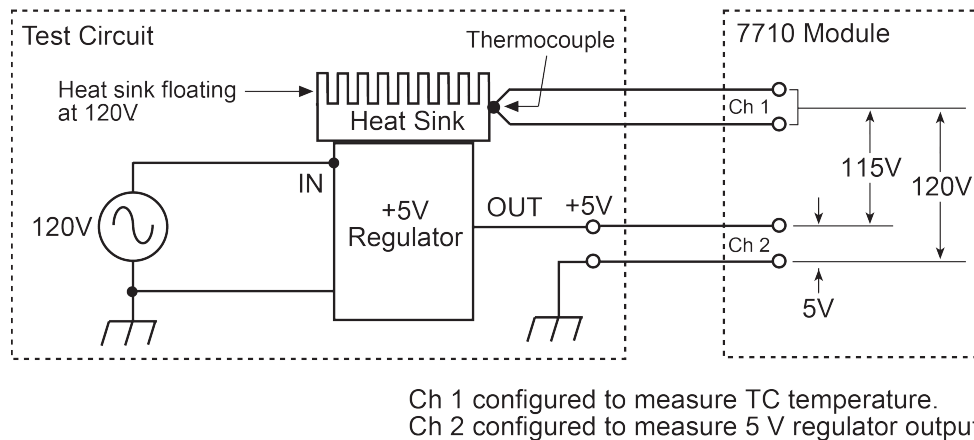
Figure 12: Example of an unsafe measurement practice
