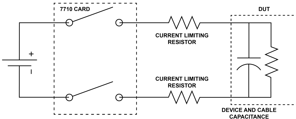
Figure 13: Solid state relay limiting resistor
