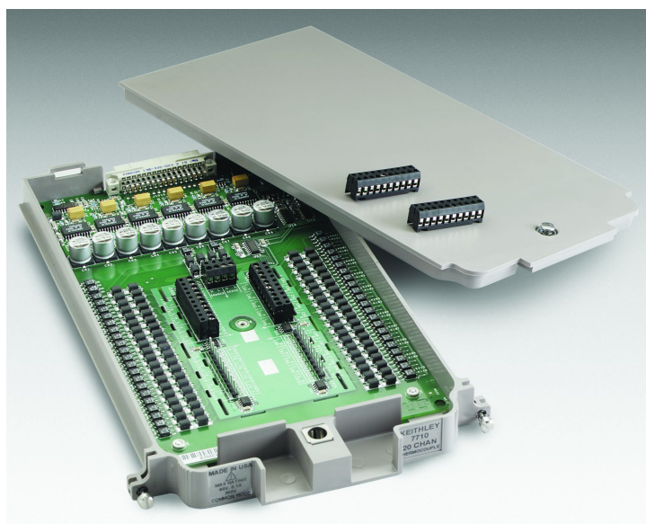
Figure 1: 7710 20-Channel Differential Multiplexer Module
