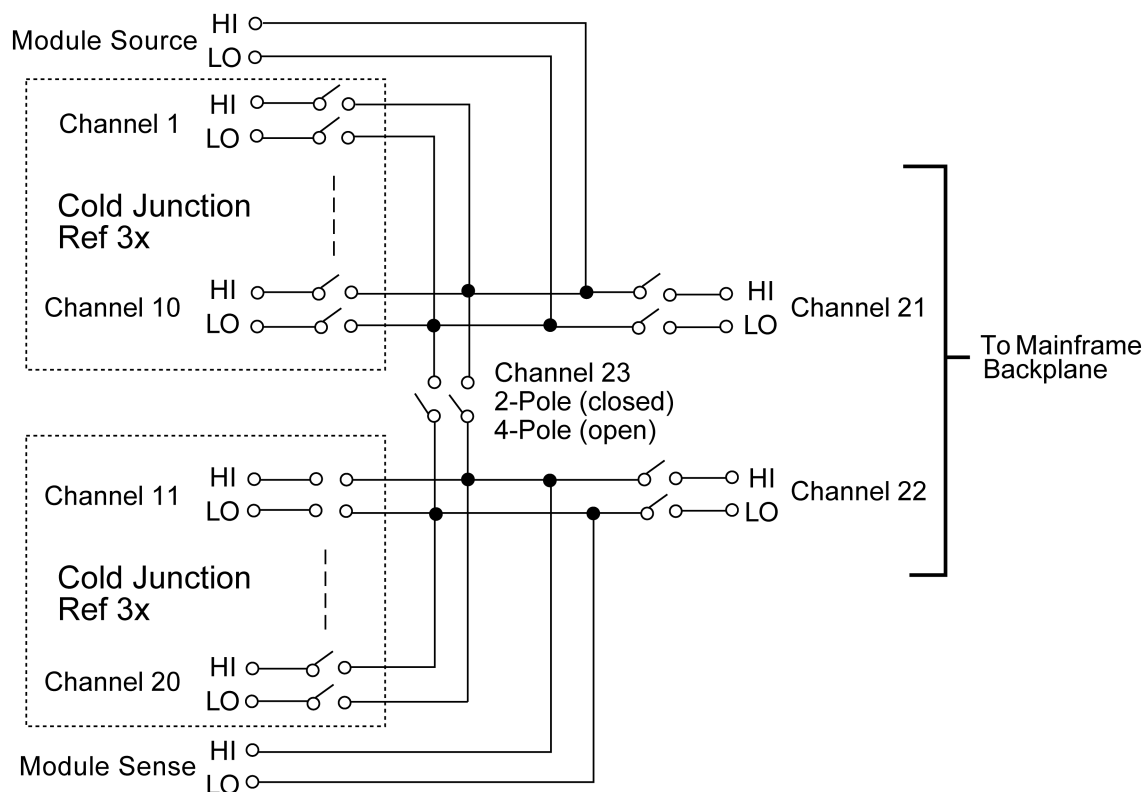
Figure 6: 7710 simplified schematic
