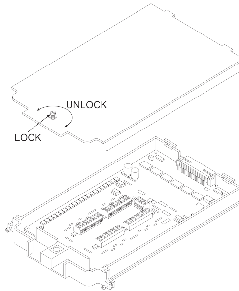
Figure 2: Screw terminal access
