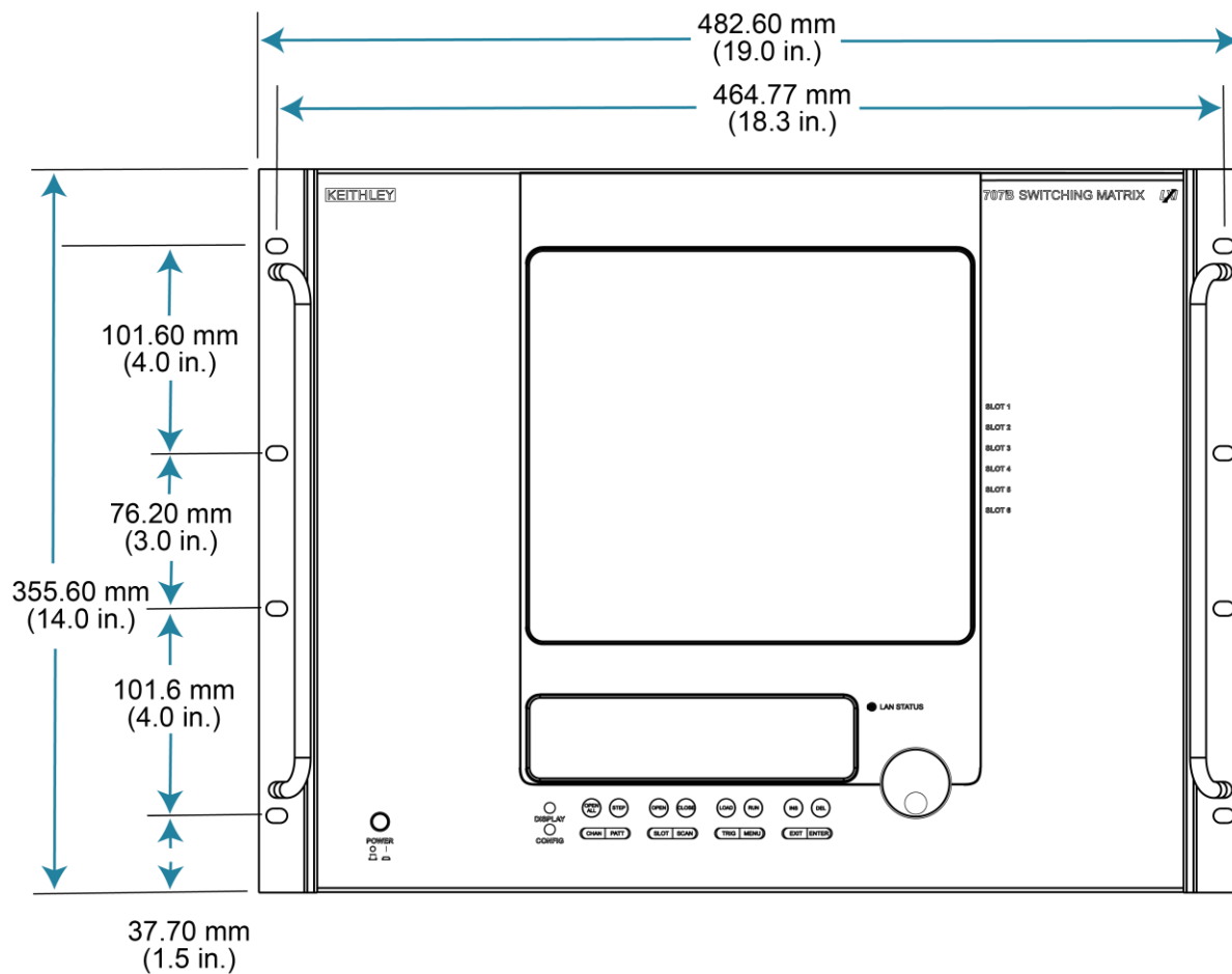
Figure 3: Dimensions - 707B front view
