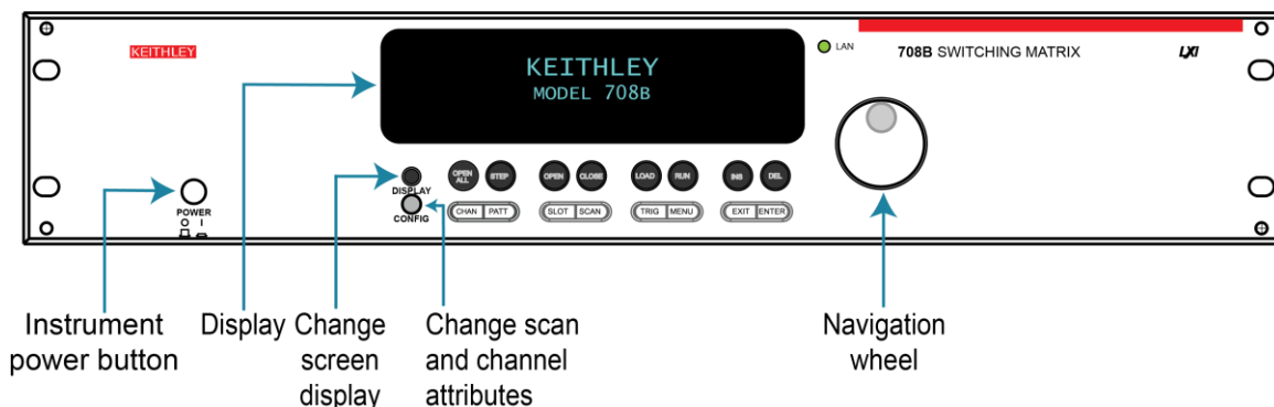
Figure 10: 708B front panel
