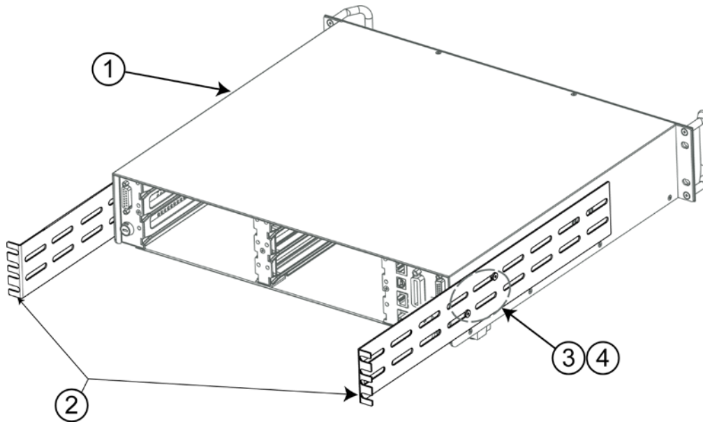
Figure 2: Rear support bracket installation
