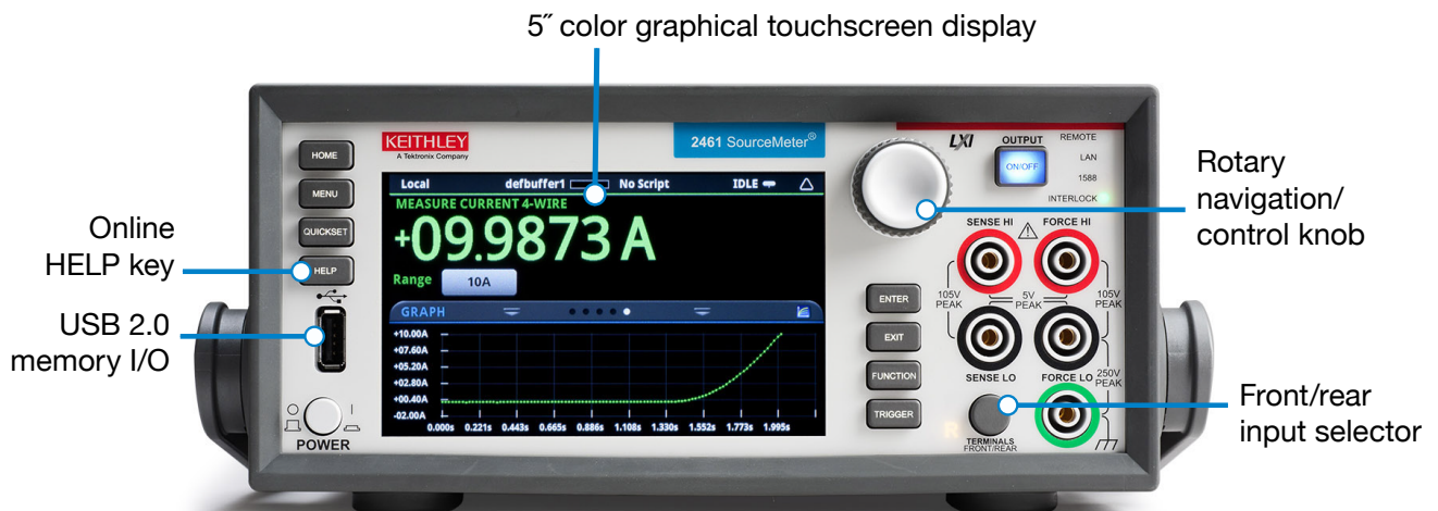
The 2461's high resolution, capacitive touchscreen and front panel controls allow for intuitive operation, even by novice users.
