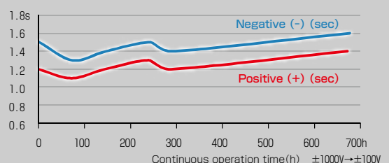
Decay Time(F-120R)
