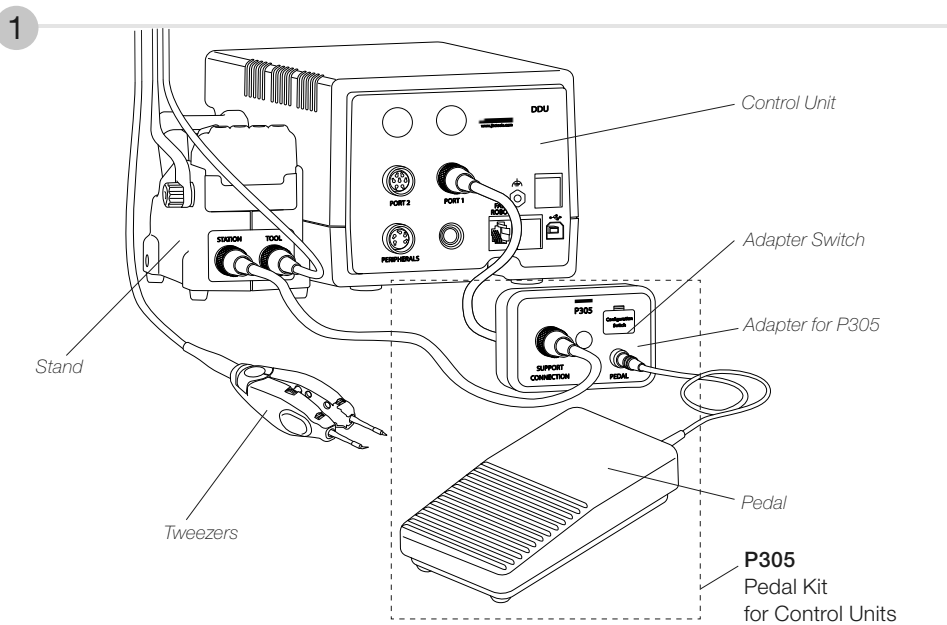
Adapter Switch
